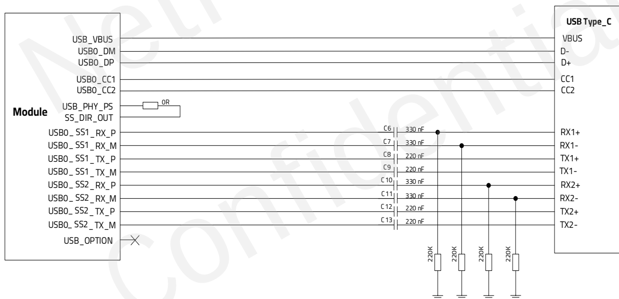
Figure 12: USB Type-C Reference Circuit of USB0
