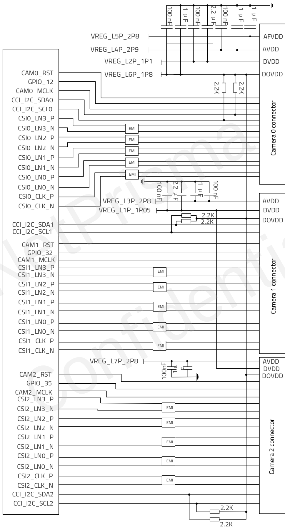
Figure 26: Reference Circuit for Three-Camera Applications
