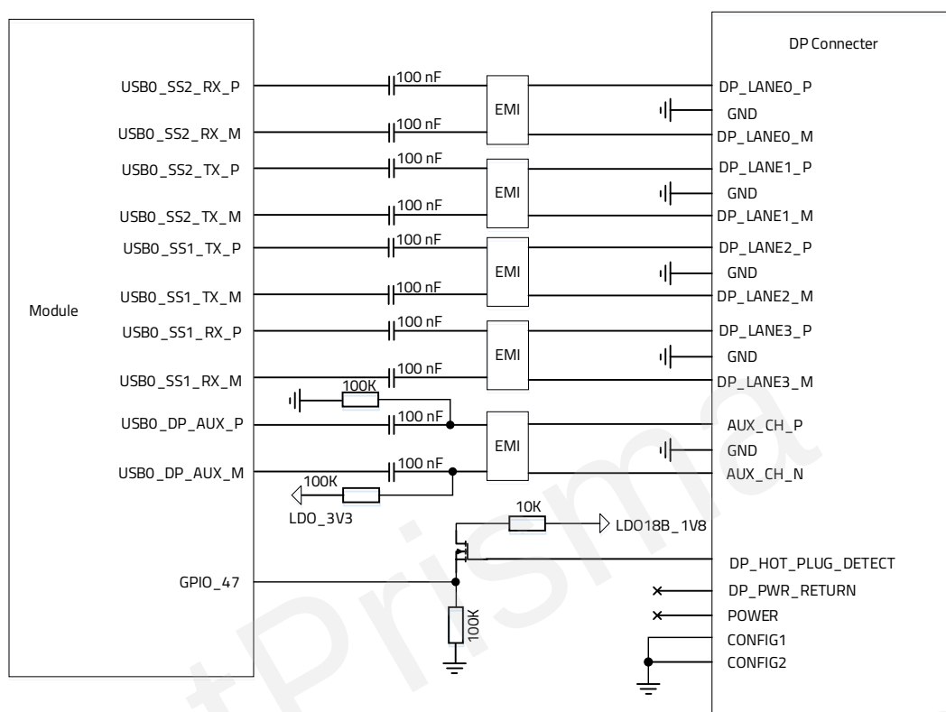
Figure 15: Standard DisplayPort Reference Circuit
