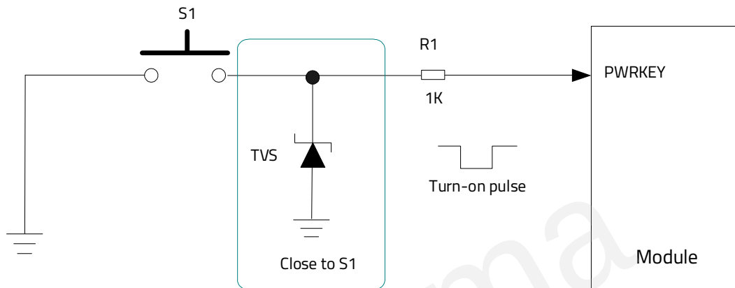
Figure 7: Turn On the Module Using Push Button
