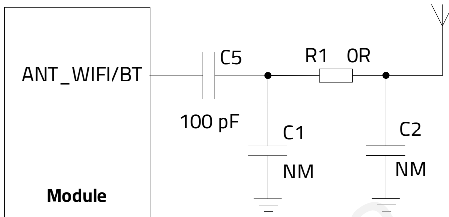
Figure 31: Reference Circuit for Wi-Fi/Bluetooth Antenna
