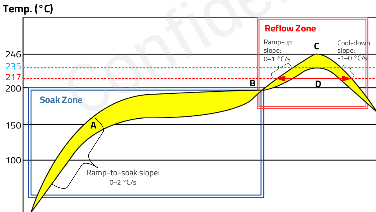
Figure 44: Recommended Reflow Soldering Thermal Profile
