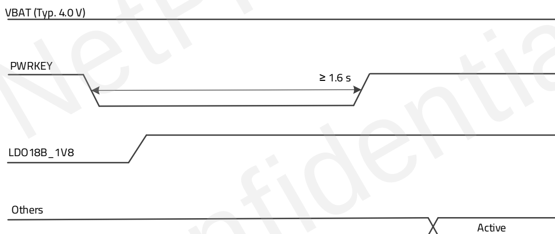
Figure 8: Turn-on Timing
