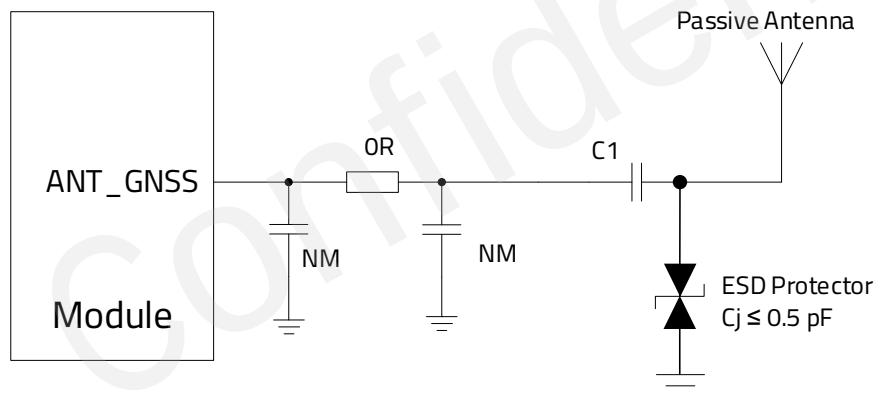
Figure 29: Reference Circuit for Passive Antenna
