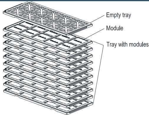
Figure 46: Packaging Process
