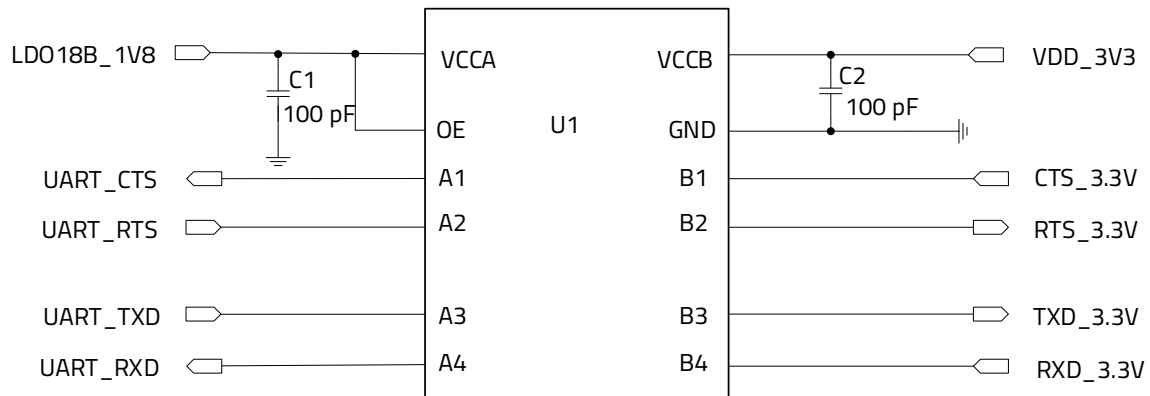
Figure 20: Reference Circuit with Level-Shifting Chip (for UART)
