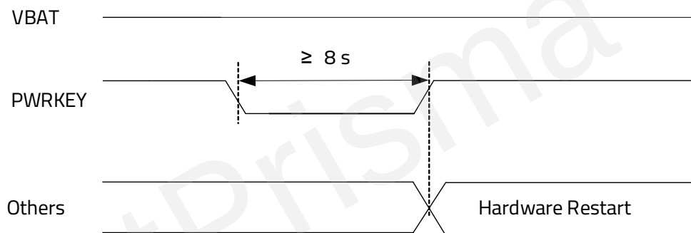
Figure 9: Restart Timing
