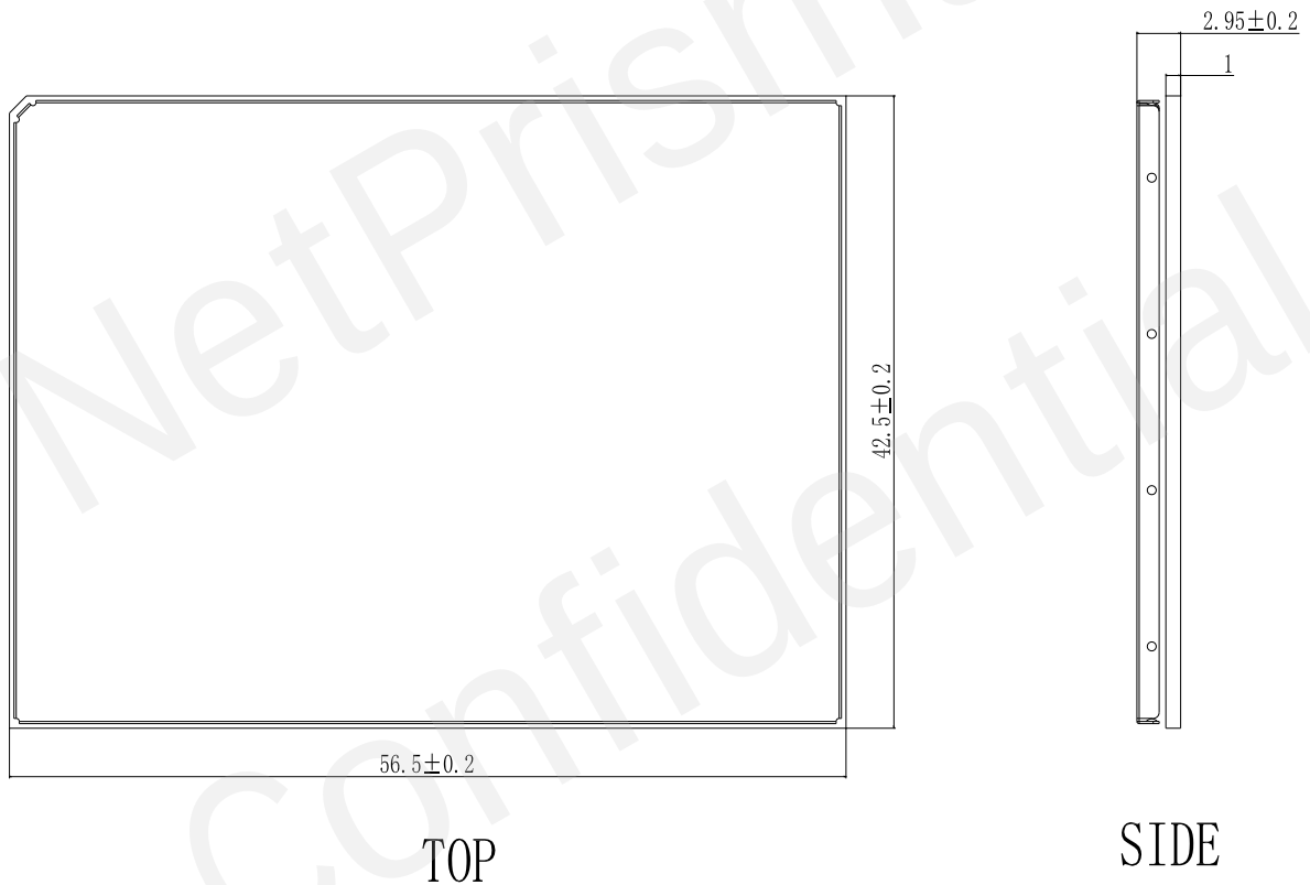
Figure 40: Module Top and Side Dimensions
