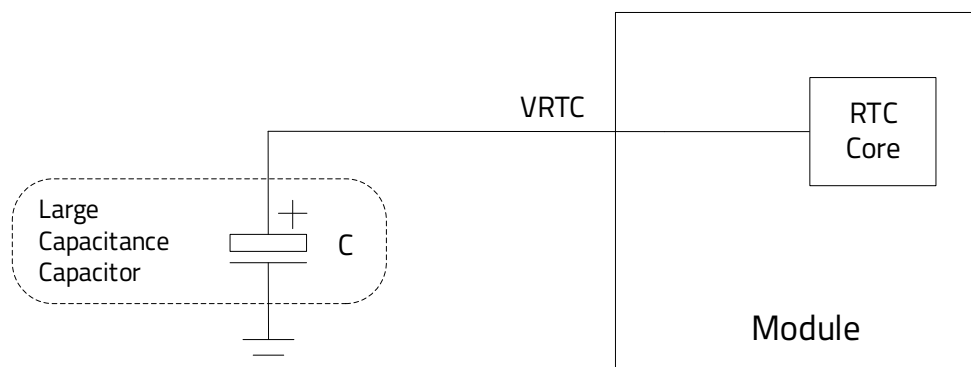
Figure 11: RTC Powered by Capacitor
