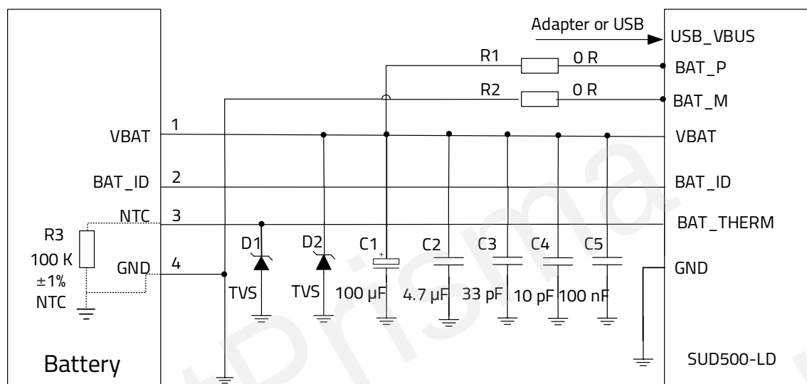
Figure 2: Reference Design for Battery Charging Circuit
