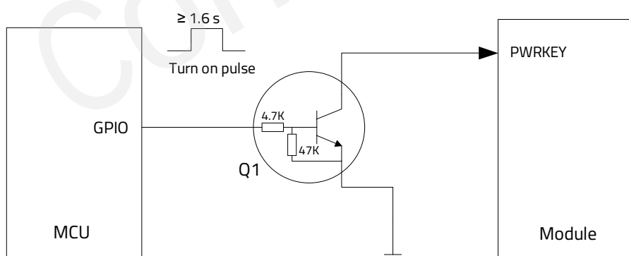
Figure 6: Turn On the Module Using Driving Circuit
