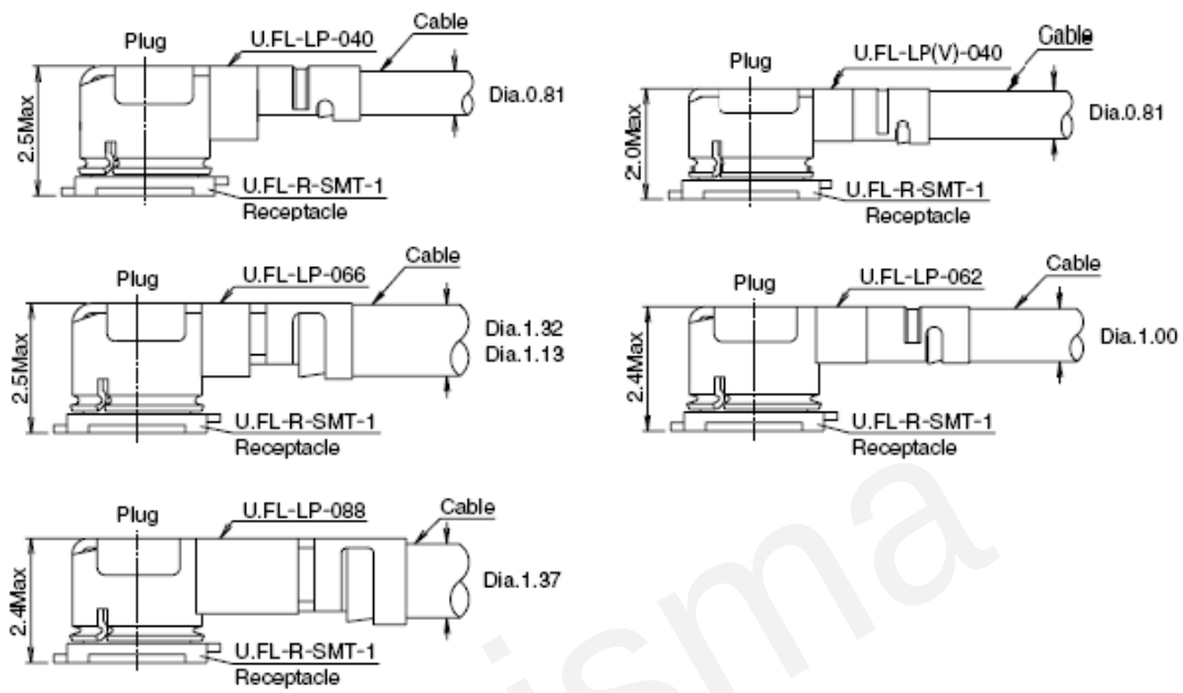
Figure 39: Space Factor of Mated Connectors (Unit: mm)
