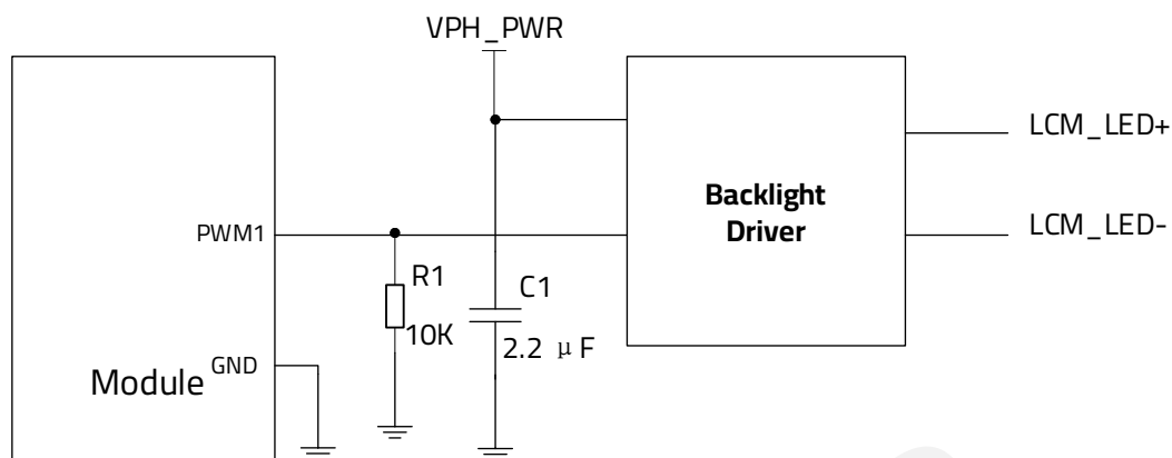
Figure 23: LCM External Backlight Driver Reference Circuit
