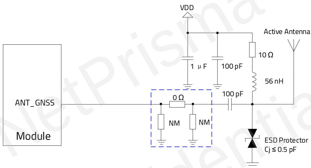
Figure 30: Reference Circuit for Active Antenna
