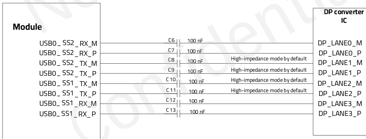
Figure 16: Reference Design for External DP Converter IC
