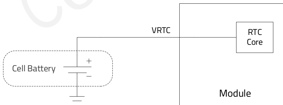
Figure 10: RTC Powered by a Rechargeable Cell Battery
