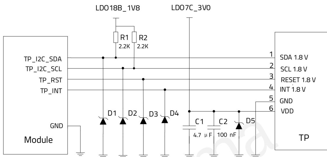
Figure 24: Reference Circuit for TP Interface
