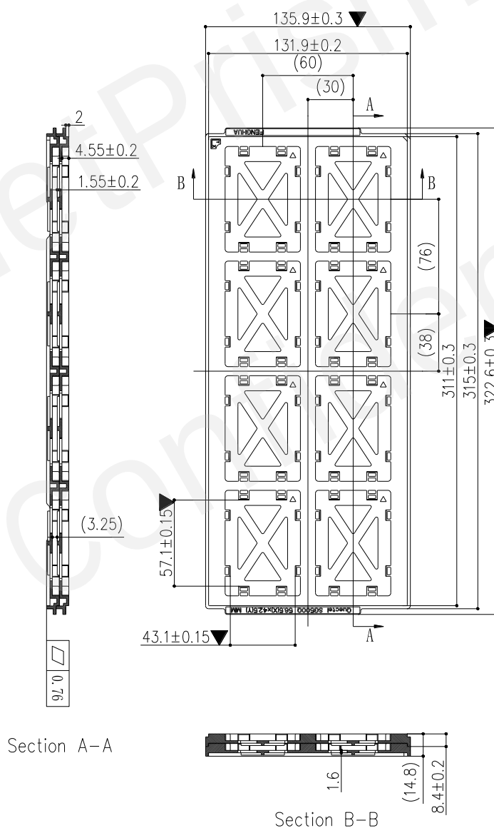
Figure 45: Injection Tray Dimension Drawing (Unit: mm)
