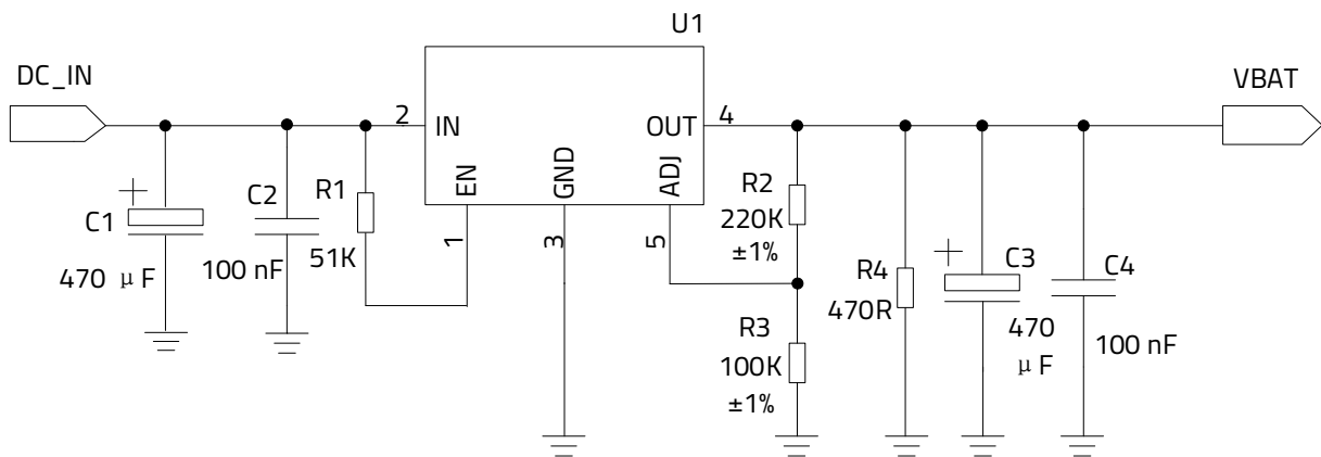
Figure 3: Reference Design for Power Supply
