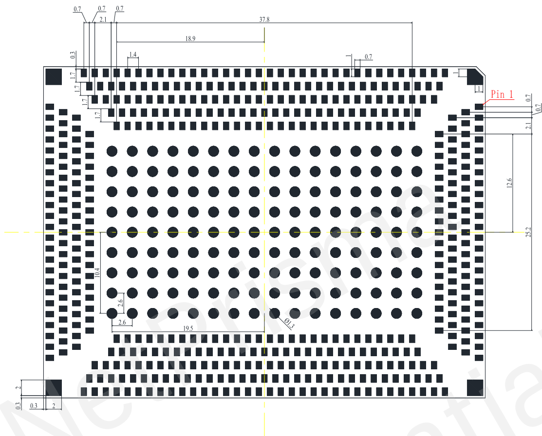
Figure 4 1: Module Bottom Dimensions (Bottom View)
