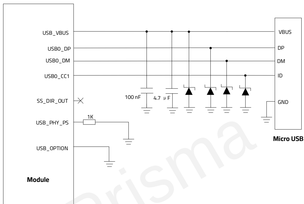
Figure 13: Micro USB Reference Circuit of USB0
