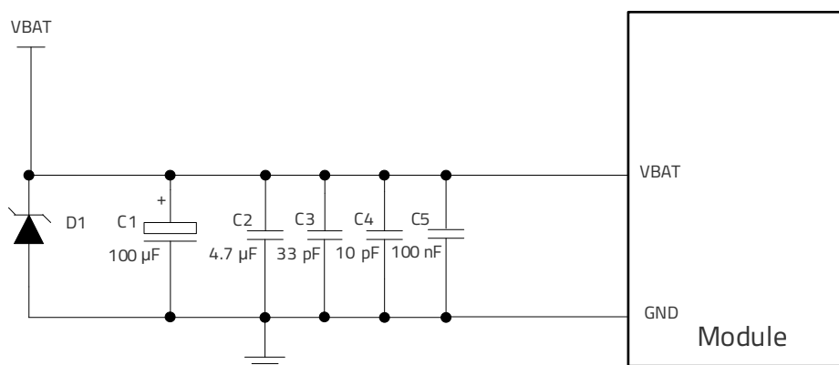
Figure 5: Structure of Power Supply
