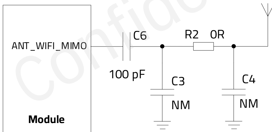
Figure 32: Reference Circuit for Wi-Fi MIMO Antenna
