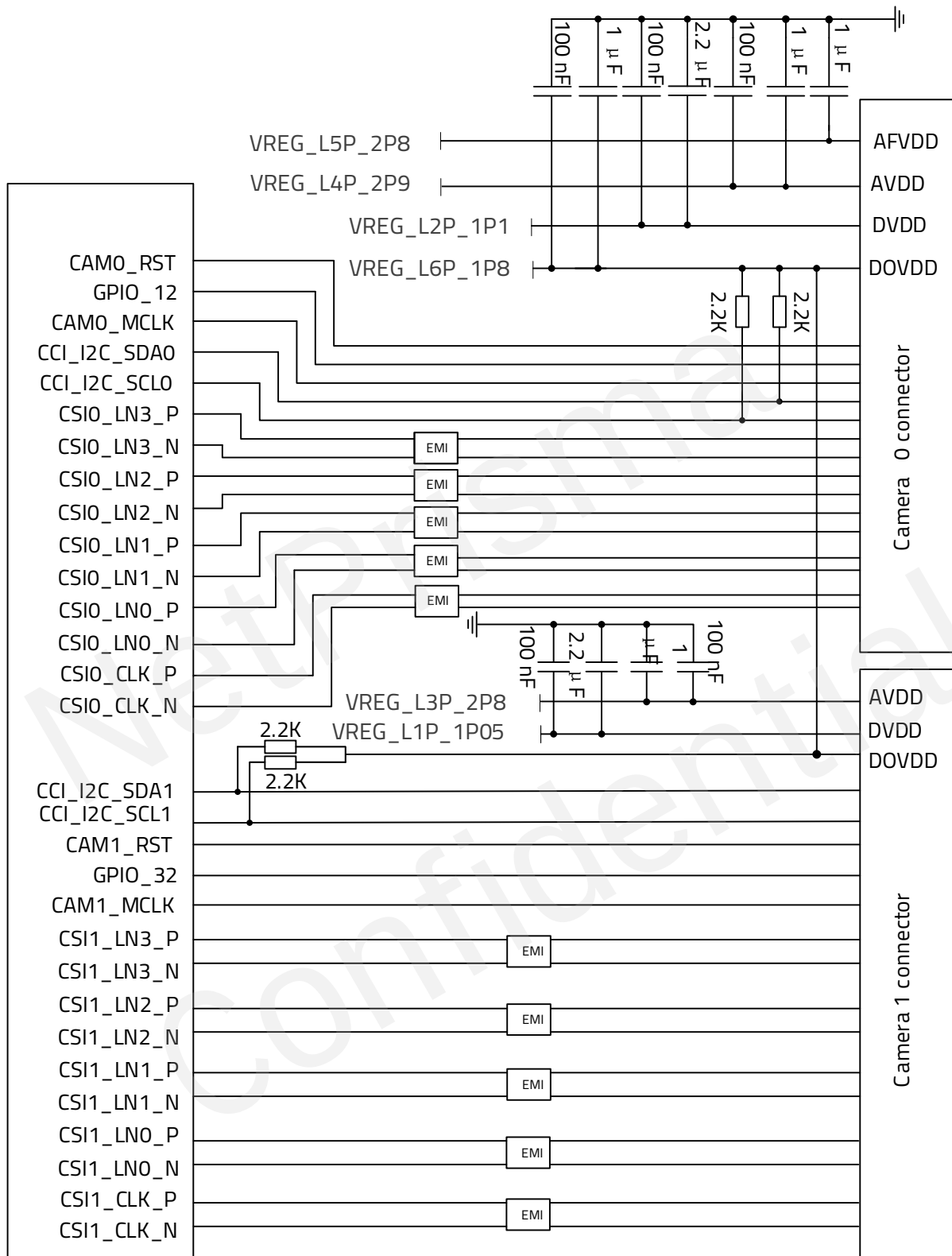
Figure 25: Reference Circuit for Dual-Camera Applications
