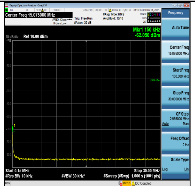
Band26(824-849)-15MHz-QPSK-26965-1RB#0-0.15~30- PASS
