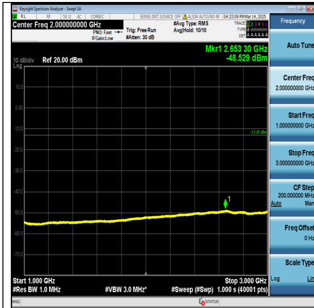
Band26(824-849)-15MHz-QPSK-26915-1RB#0- 1000~3000-PASS
