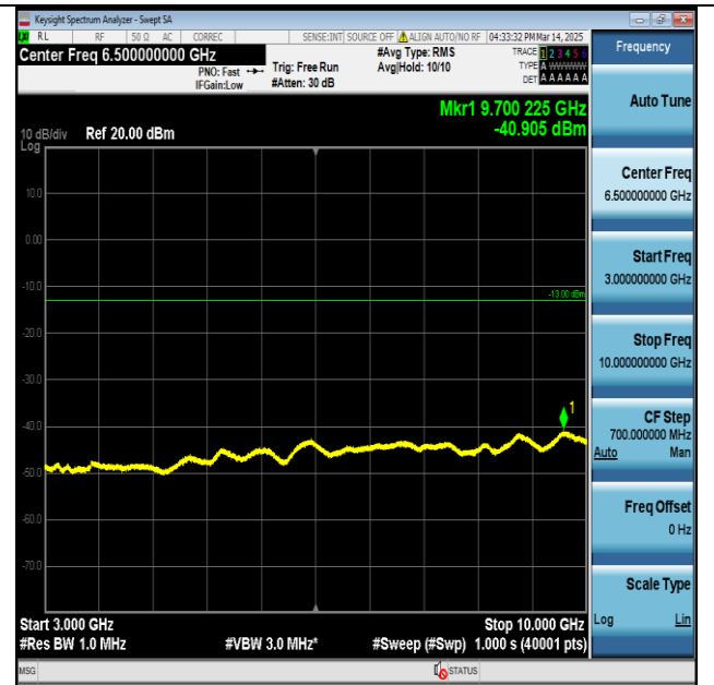
Band26(824-849)-15MHz-QPSK-26915-1RB#0- 3000~10000-PASS
