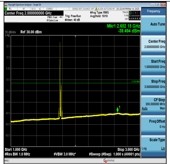
Band66-20MHz-QPSK-132572-1RB#0-1000~3000-PASS
