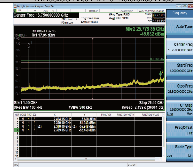
11n40SISO-Ant0-2422-1000-26500-PASS
