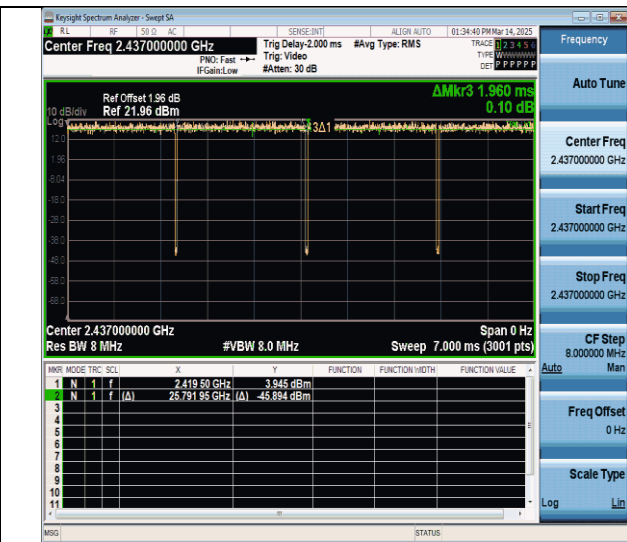
NTNV-11n20SISO-Ant0-2437
