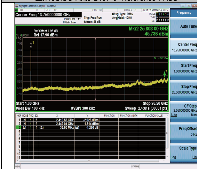
11n40SISO-Ant0-2437-1000-26500-PASS
