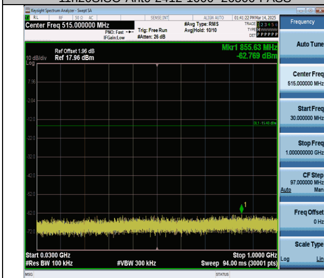
11n20SISO-Ant0-2437-30-1000-PASS
