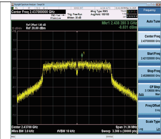
11n20SISO-Ant0-2437-PASS
