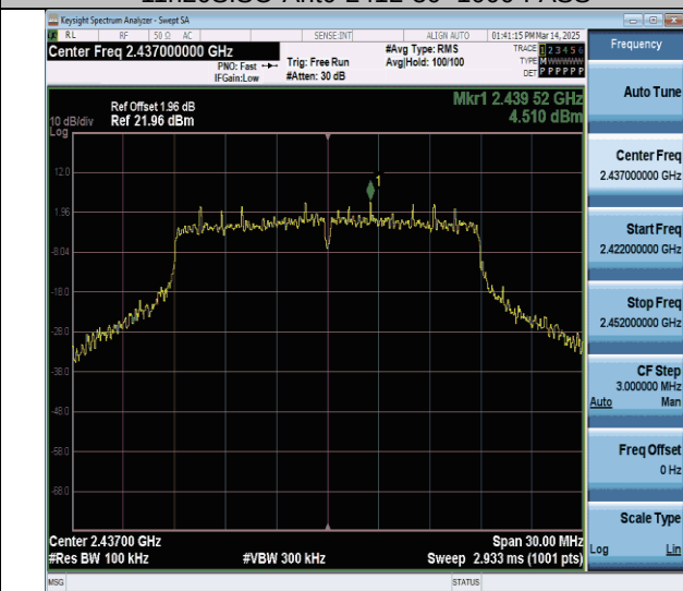
11n20SISO-Ant0-2437-0-Reference-PASS
