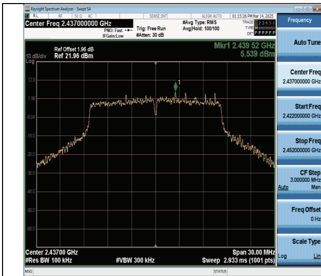
11g-Ant0-2437-0~Reference-PASS
