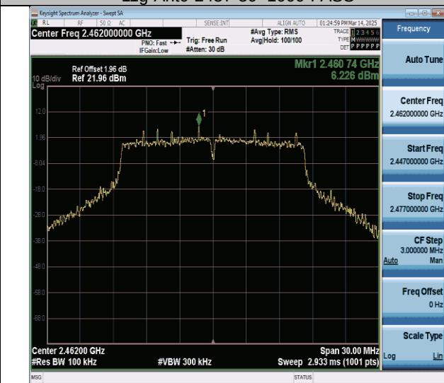
11g-Ant0-2462-0~Reference-PASS
