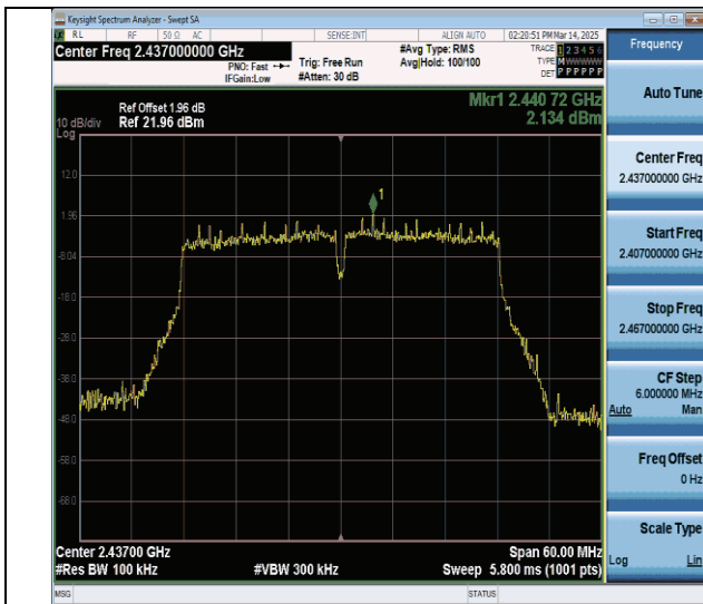
11n40SISO-Ant0-2437-0-Reference-PASS
