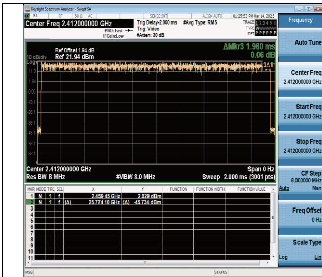
NTNV-11n20SISO-Ant0-2412
