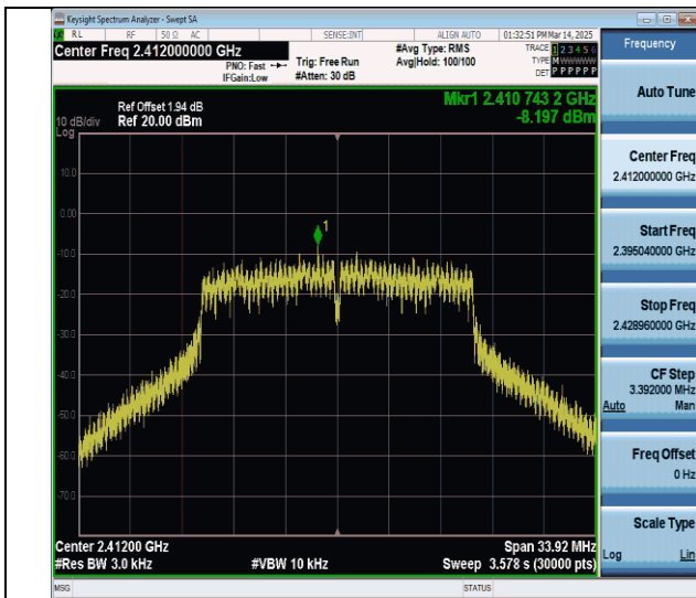
11n20SISO-Ant0-2412-PASS
