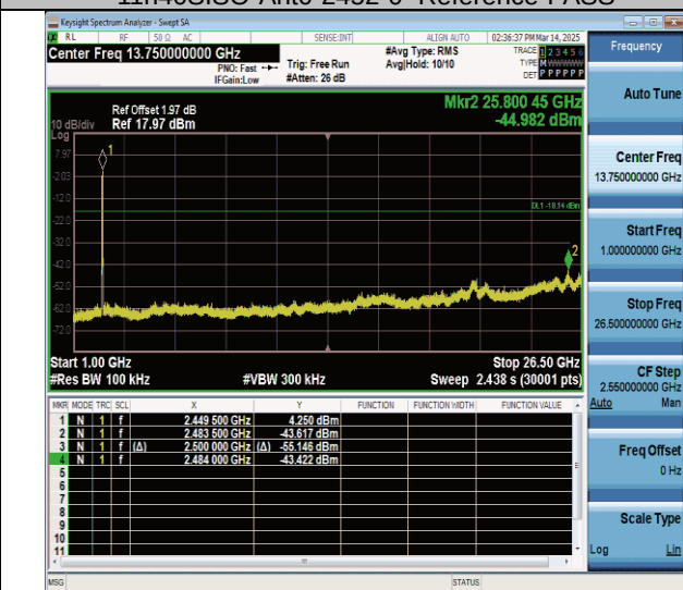
11n40SISO-Ant0-2452-1000-26500-PASS
