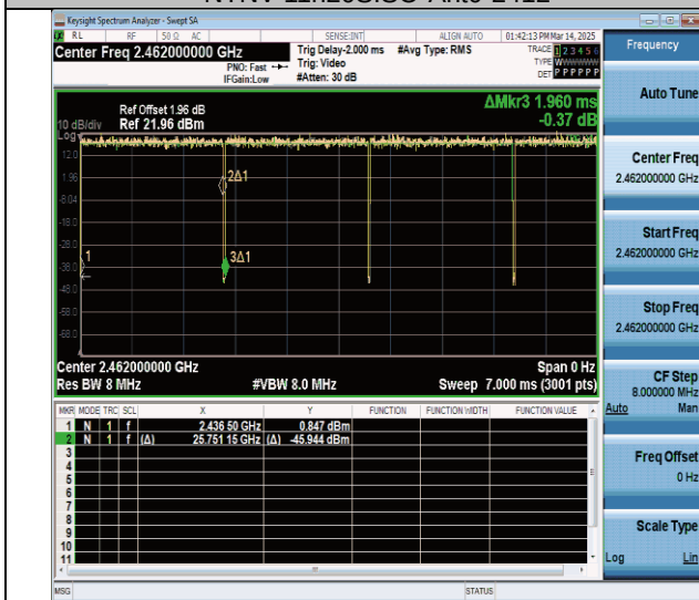
NTNV-11n20SISO-Ant0-2462
