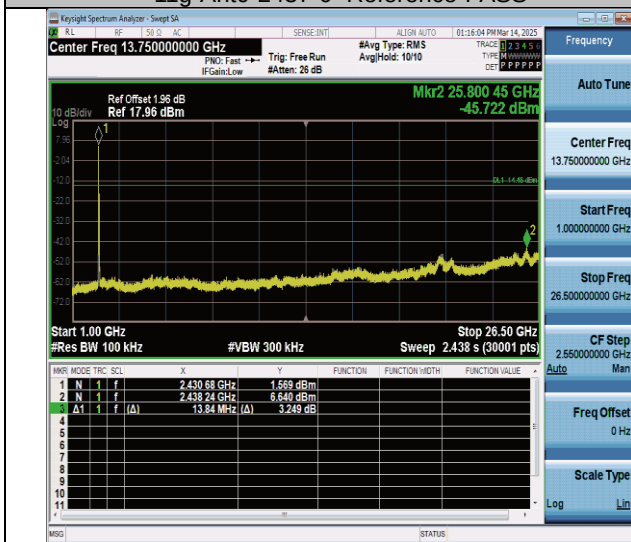
11g-Ant0-2437-1000~26500-PASS
