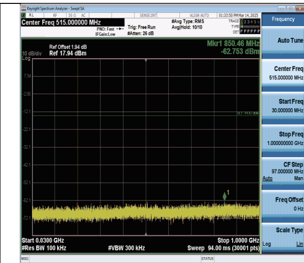
11n20SISO-Ant0-2412-30-1000-PASS
