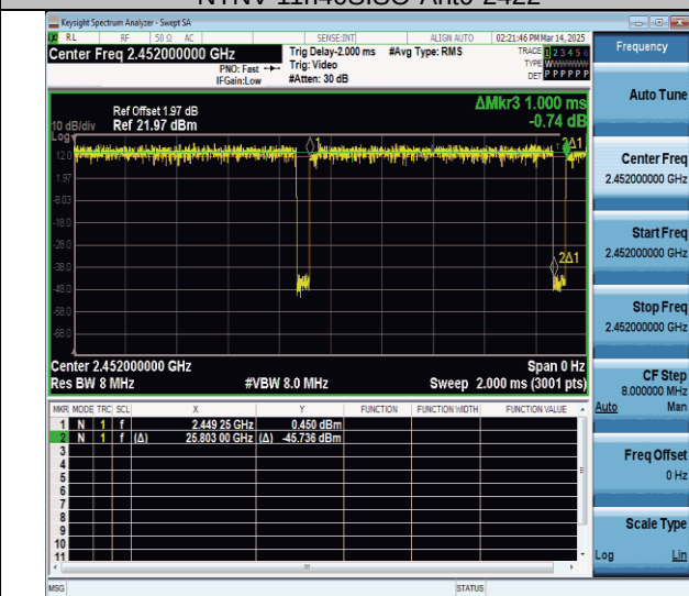
NTNV-11n40SISO-Ant0-2452
