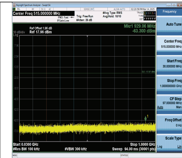
11n40SISO-Ant0-2437-30-1000-PASS
