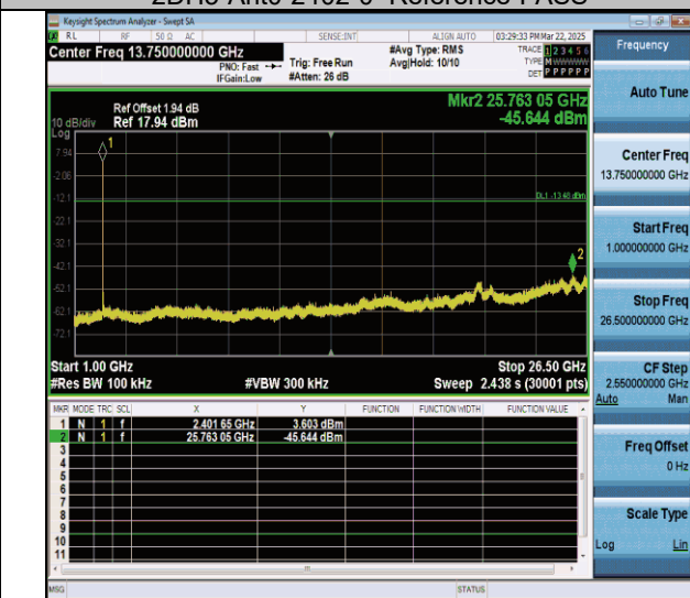
2DH5-Ant0-2402-1000~26500-PASS
