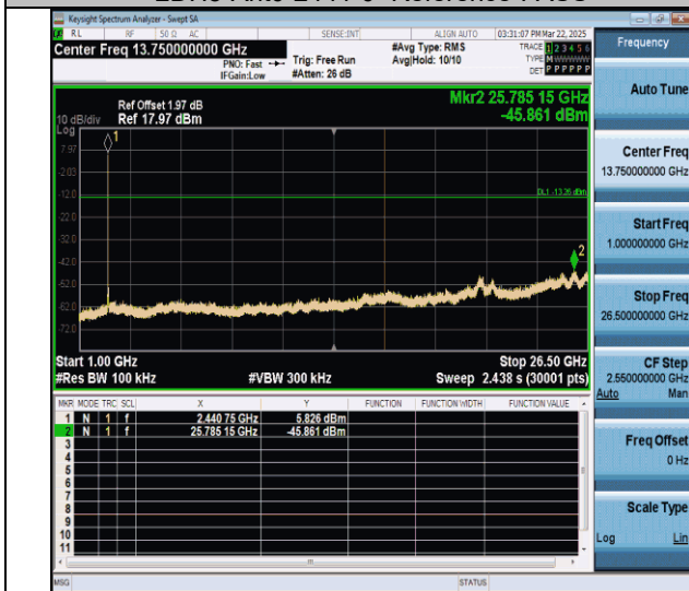
2DH5-Ant0-2441-1000~26500-PASS
