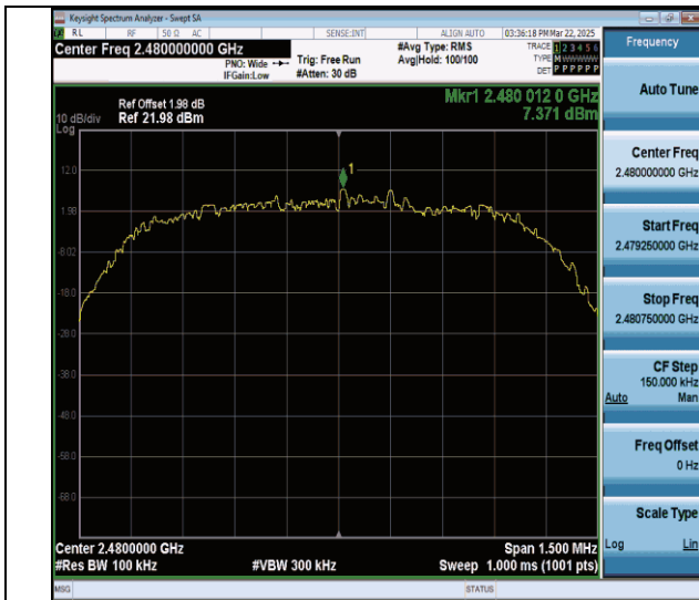
3DH5-Ant0-2480-0~Reference-PASS
