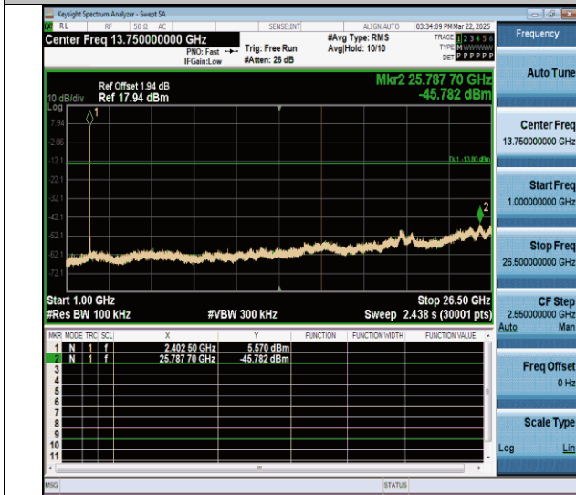
3DH5-Ant0-2402-1000~26500-PASS
