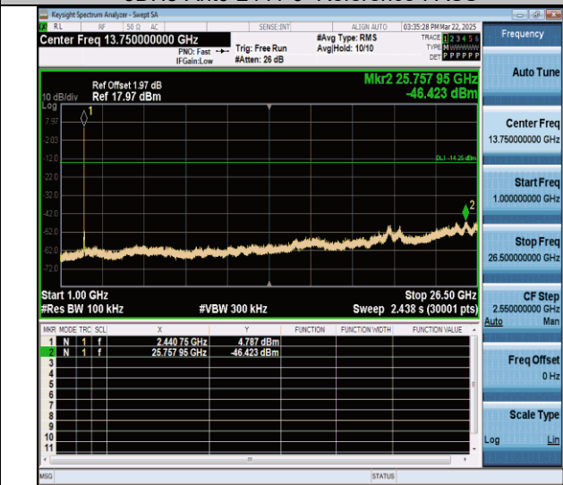
3DH5-Ant0-2441-1000~26500-PASS
