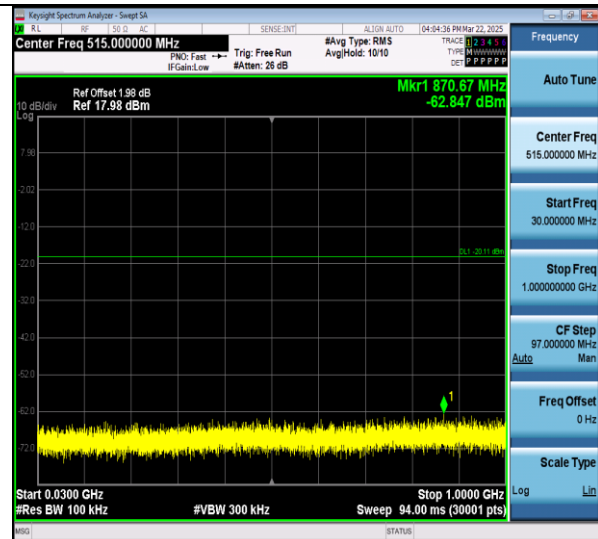
BLE_1M-Ant0-2480-30~1000-PASS
