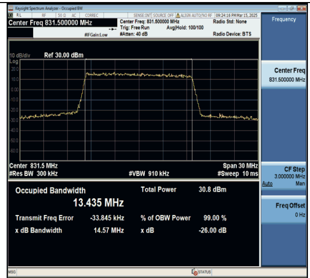
Band26(824-849)-15MHz-16QAM-26865-75RB#0-PASS
