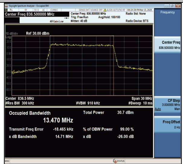
Band26(824-849)-15MHz-16QAM-26915-75RB#0-PASS
