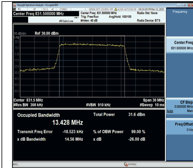
Band26(824-849)-15MHz-QPSK-26865-75RB#0-PASS
