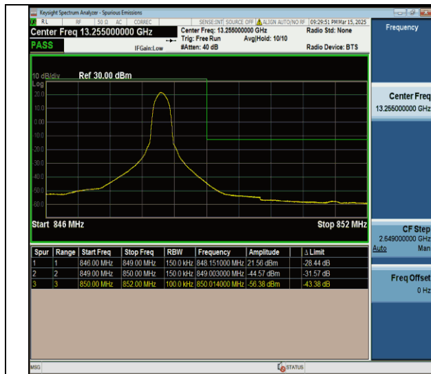
Band26(824-849)-15MHz-QPSK-26965-1RB#74-PASS
