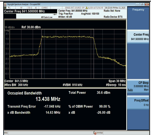
Band26(824-849)-15MHz-16QAM-26965-75RB#0-PASS
