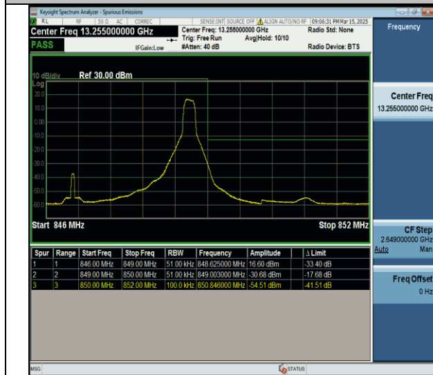
Band26(824-849)-5MHz-QPSK-27015-1RB#24-PASS
