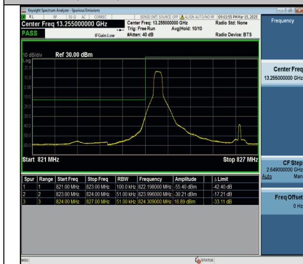
Band26(824-849)-5MHz-QPSK-26815-1RB#0-PASS
