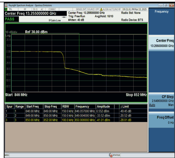
Band26(824-849)-15MHz-QPSK-26965-75RB#0-PASS
