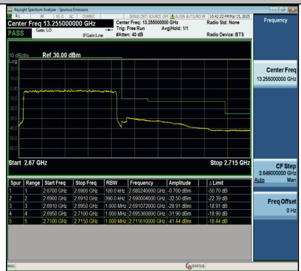
Band41-20MHz-QPSK-41490-100RB#0-PASS
