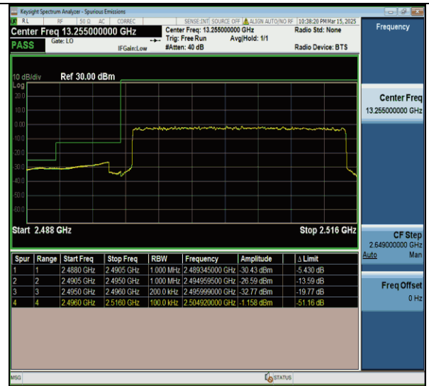
Band41-20MHz-QPSK-39750-100RB#0-PASS
