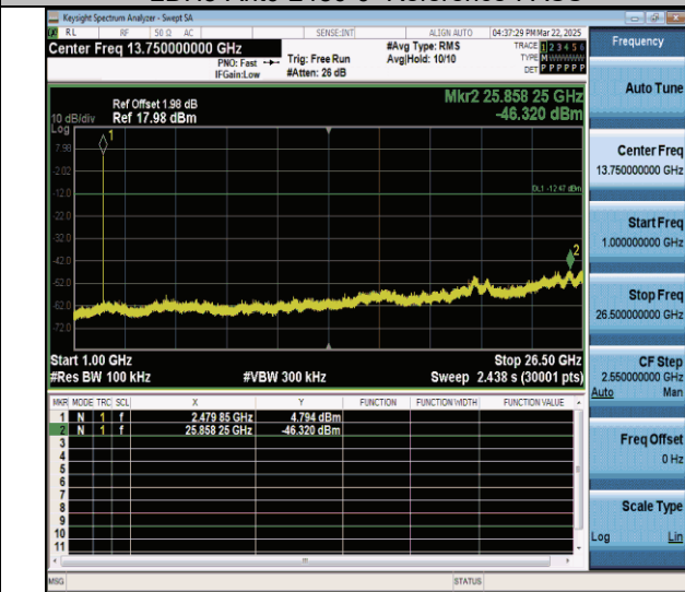
2DH5-Ant0-2480-1000~26500-PASS
