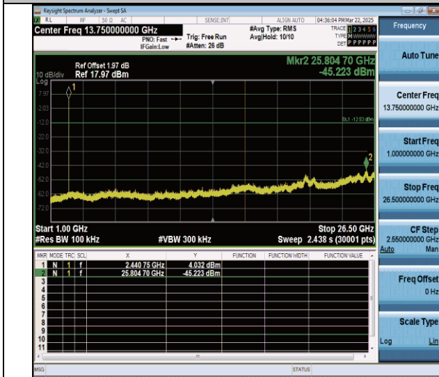
2DH5-Ant0-2441-1000~26500-PASS
