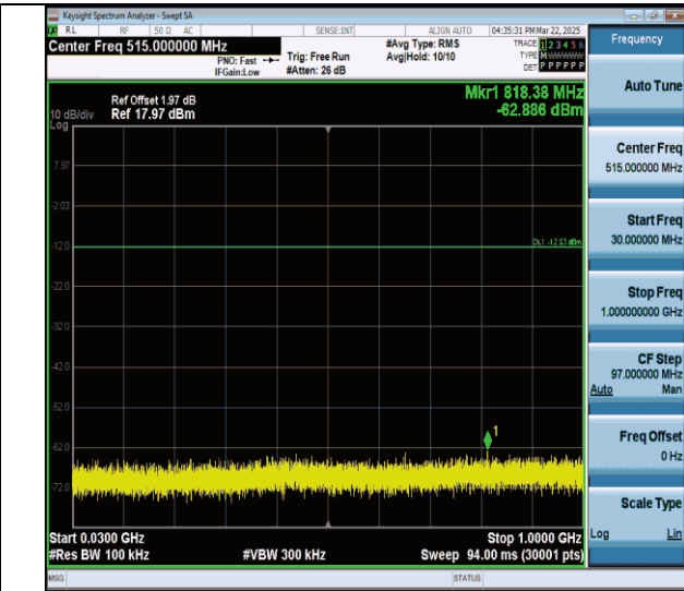
2DH5-Ant0-2441-30~1000-PASS
