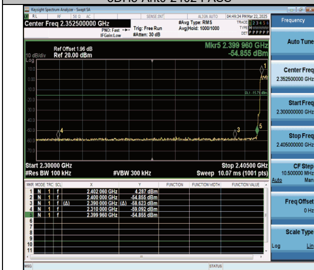
3DH5-Ant0-Hop 2402-PASS
