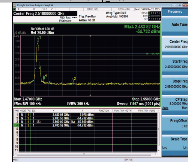
3DH5-Ant0-2480-PASS
