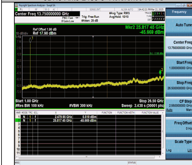
3DH5-Ant0-2480-1000~26500-PASS
