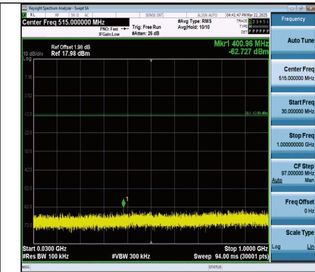
3DH5-Ant0-2480-30~1000-PASS
