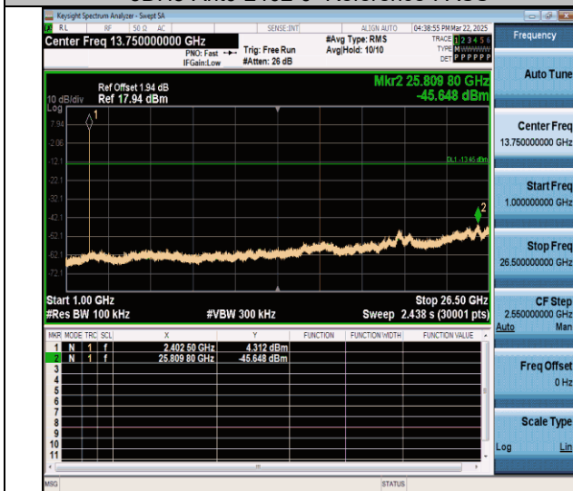
3DH5-Ant0-2402-1000~26500-PASS
