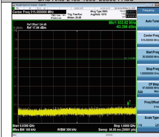
2DH5-Ant0-2402-30~1000-PASS
