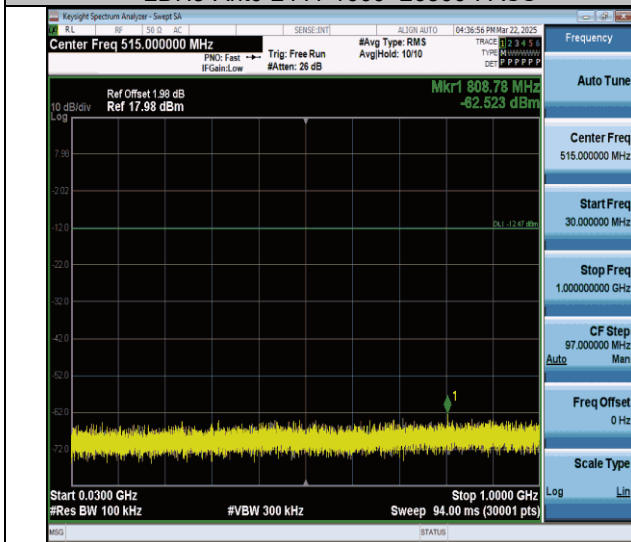
2DH5-Ant0-2480-30~1000-PASS
