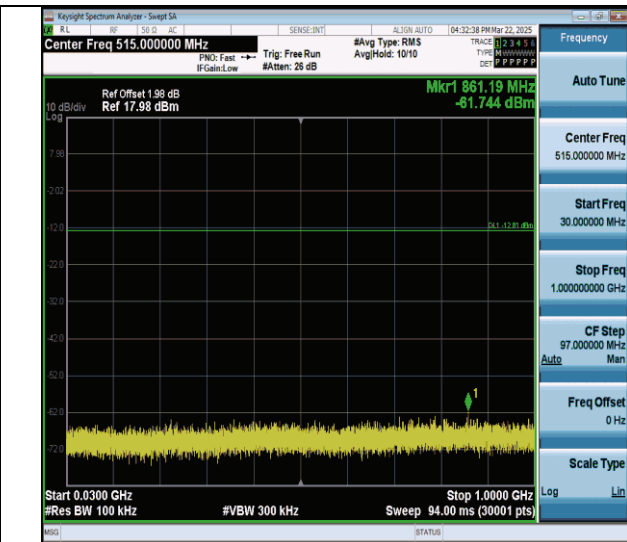
DH5-Ant0-2480-30~1000-PASS
