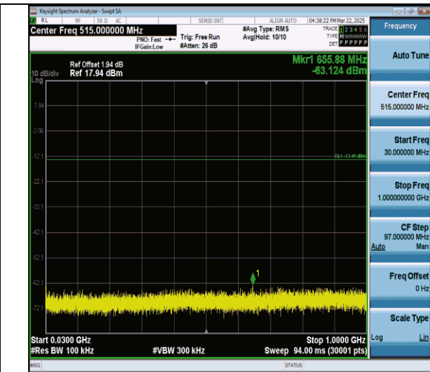
3DH5-Ant0-2402-30~1000-PASS
