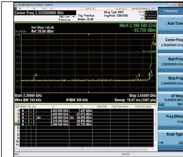
2DH5-Ant0-Hop 2402-PASS
