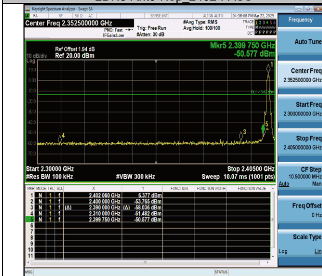
3DH5-Ant0-2402-PASS
