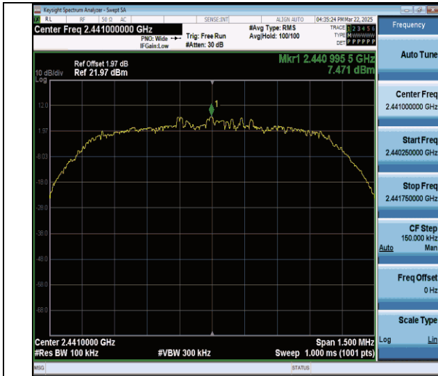
2DH5-Ant0-2441-0~Reference-PASS
