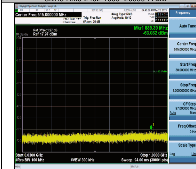
3DH5-Ant0-2441-30~1000-PASS
