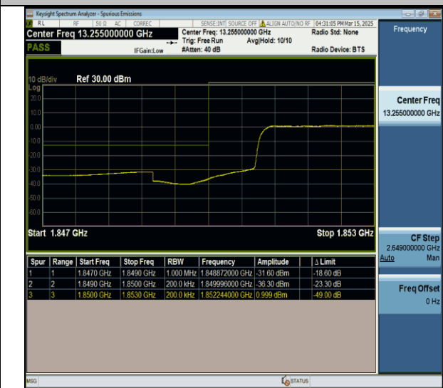
Band25-20MHz-QPSK-26140-100RB#0-PASS
