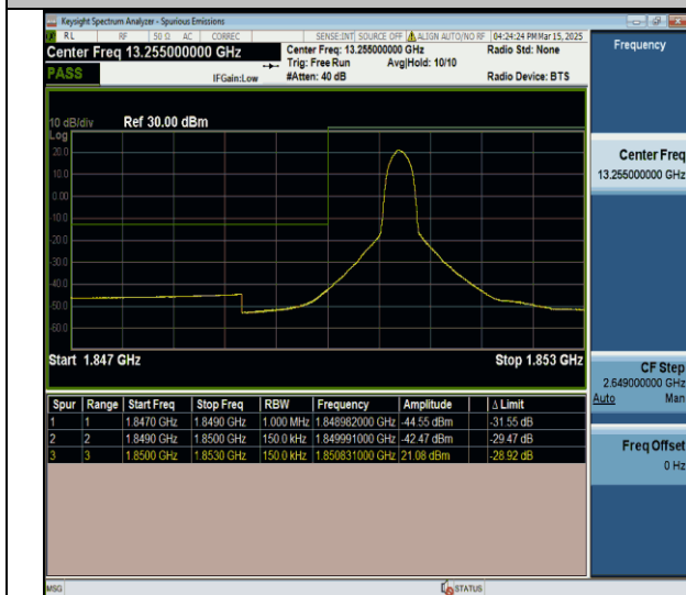
Band25-15MHz-QPSK-26115-1RB#0-PASS
