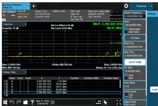
3DH5-Ant1-2402-PASS
