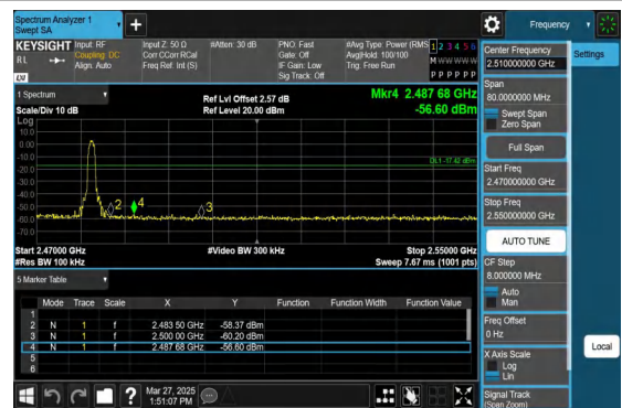
3DH5-Ant1-Hop_2480-PASS
