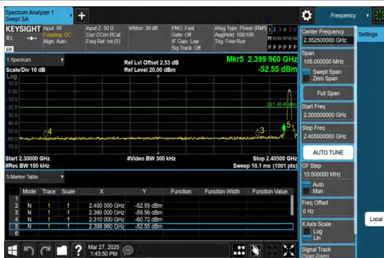
3DH5-Ant1-Hop_2402-PASS
