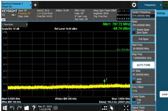
3DH5-Ant1-2402-30~1000-PASS
