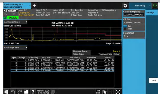
Band41-15MHz-QPSK-41515-1RB#0-PASS
