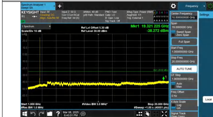
Band41-5MHz-QPSK-40620-1RB#24-1000~20000-PASS
