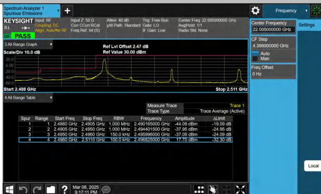
Band41-15MHz-QPSK-39725-1RB#0-PASS
