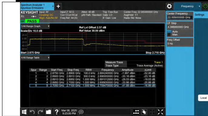
Band41-15MHz-QPSK-41515-75RB#0-PASS
