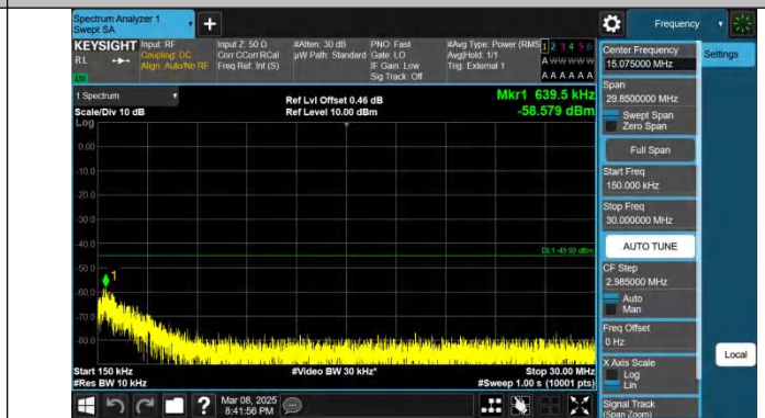
Band41-5MHz-QPSK-41565-1RB#0-0.15~30-PASS
