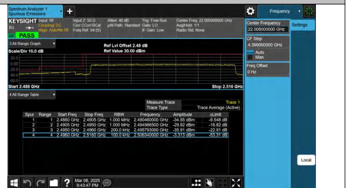
Band41-15MHz-QPSK-39750-100RB#0-PASS
