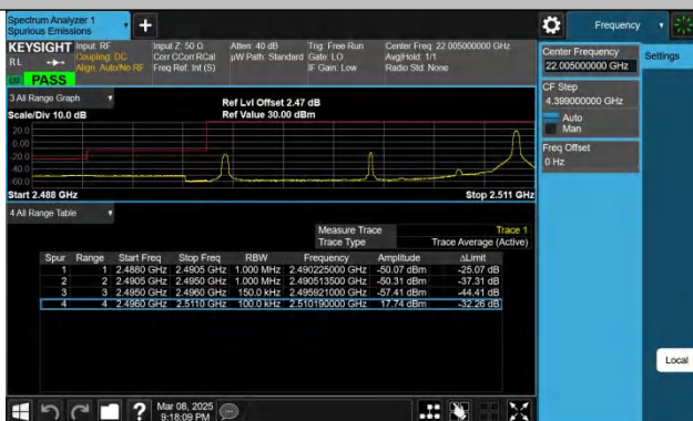
Band41-15MHz-QPSK-39725-1RB#74-PASS
