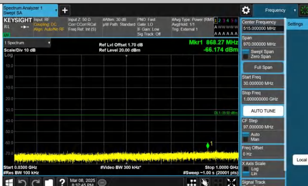
Band41-5MHz-QPSK-40620-1RB#0-30~1000-PASS
