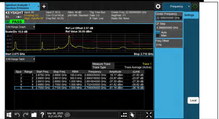
Band41-15MHz-QPSK-41515-1RB#74-PASS
