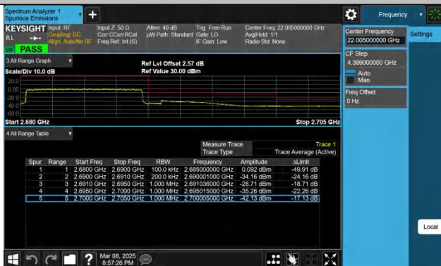
Band41-10MHz-QPSK-41540-50RB#0-PASS
