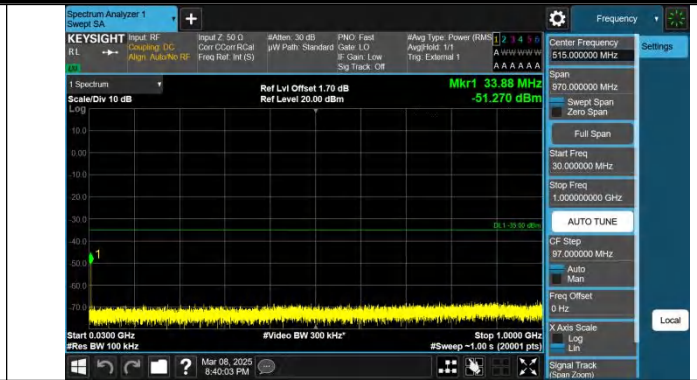
Band41-5MHz-QPSK-40620-1RB#24-30~1000-PASS
