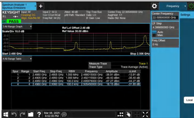
Band41-10MHz-QPSK-39700-1RB#49-PASS
