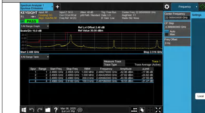
Band41-15MHz-QPSK-39750-1RB#0-PASS
