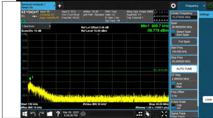
Band41-5MHz-QPSK-40620-1RB#24-0.15~30-PASS
