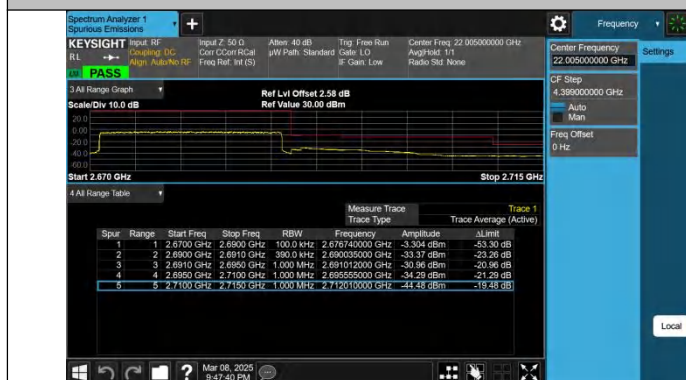
Band41-20MHz-QPSK-41490-100RB#0-PASS
