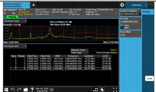
Band41-10MHz-QPSK-41540-1RB#49-PASS
