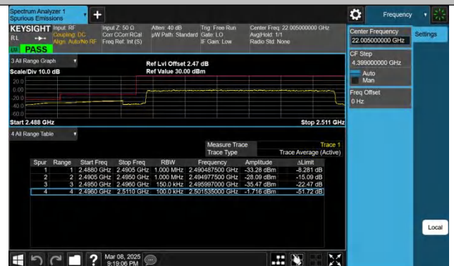
Band41-15MHz-QPSK-39725-75RB#0-PASS
