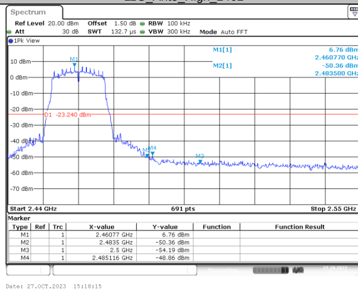
11G_Ant4_High_2462
