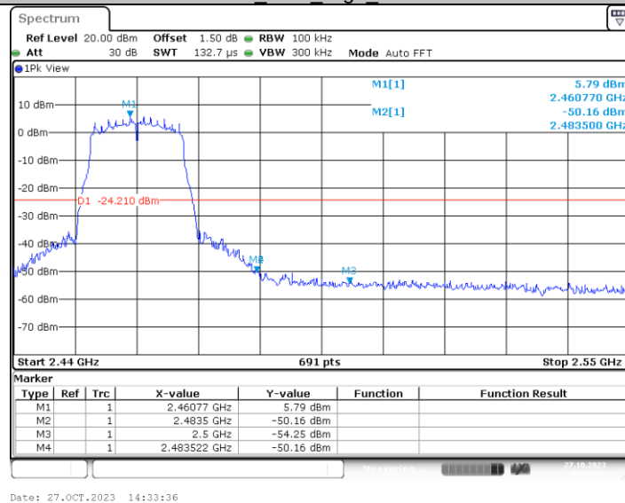
11G_Ant3_High_2462
