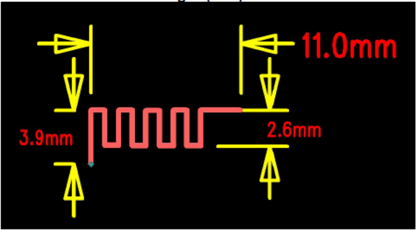
Antenna1 Photo & Length (mm)
