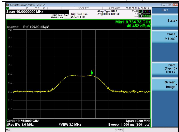
Middle channel 4 th harmonic (Peak)
