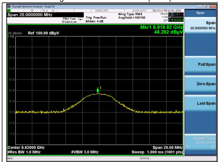
High channel 4 th harmonic (Peak)
