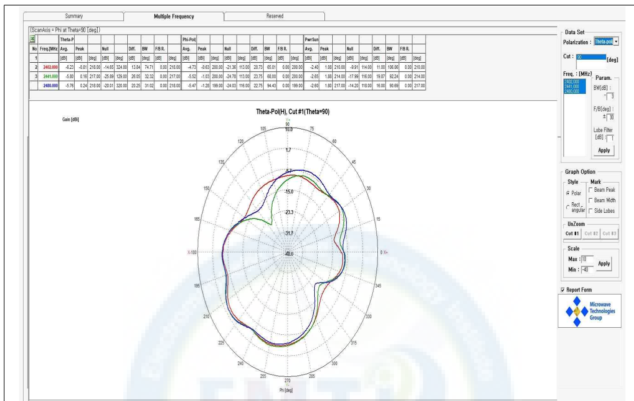
H-Cross-Pol
