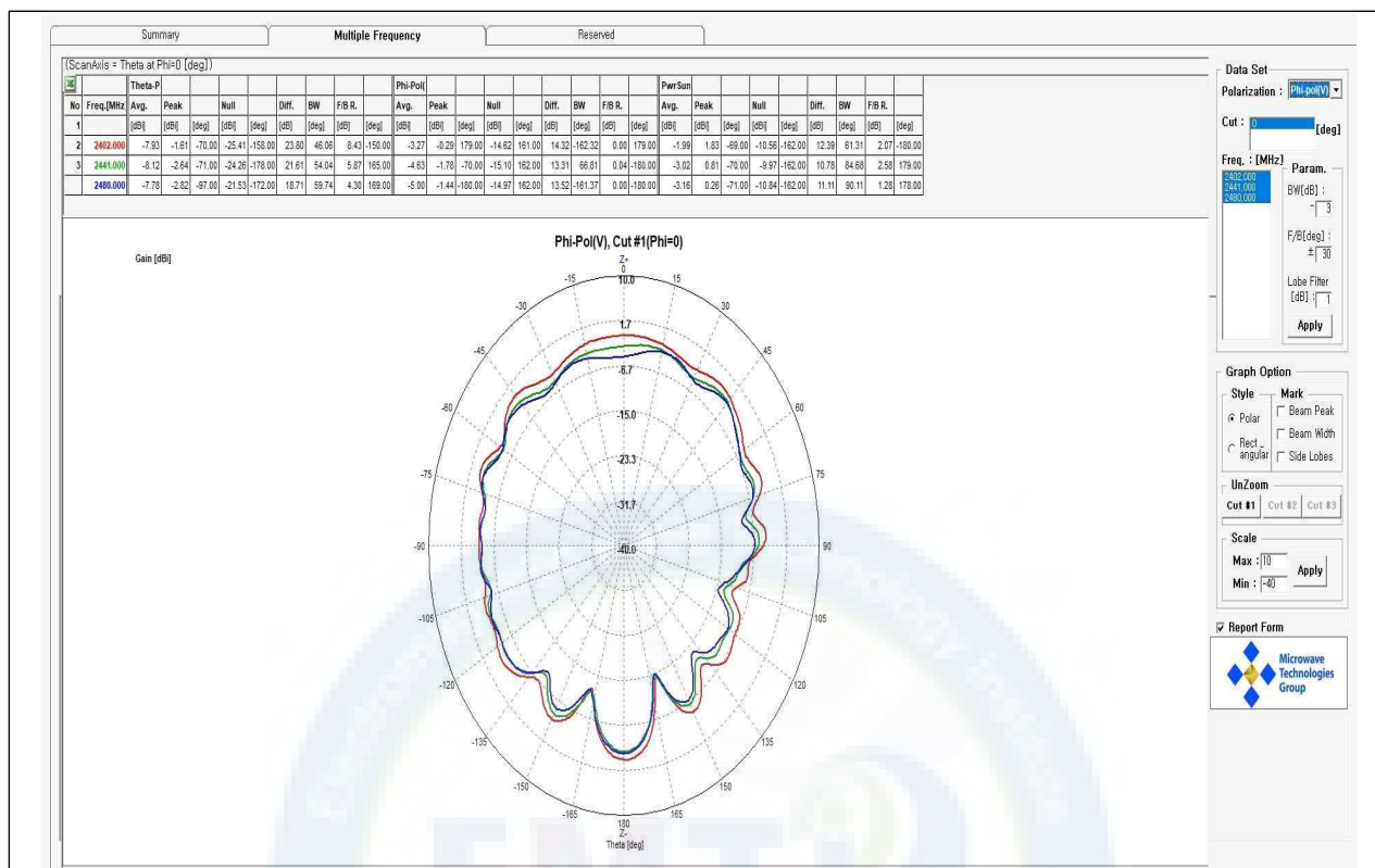
E-Co-Pol
