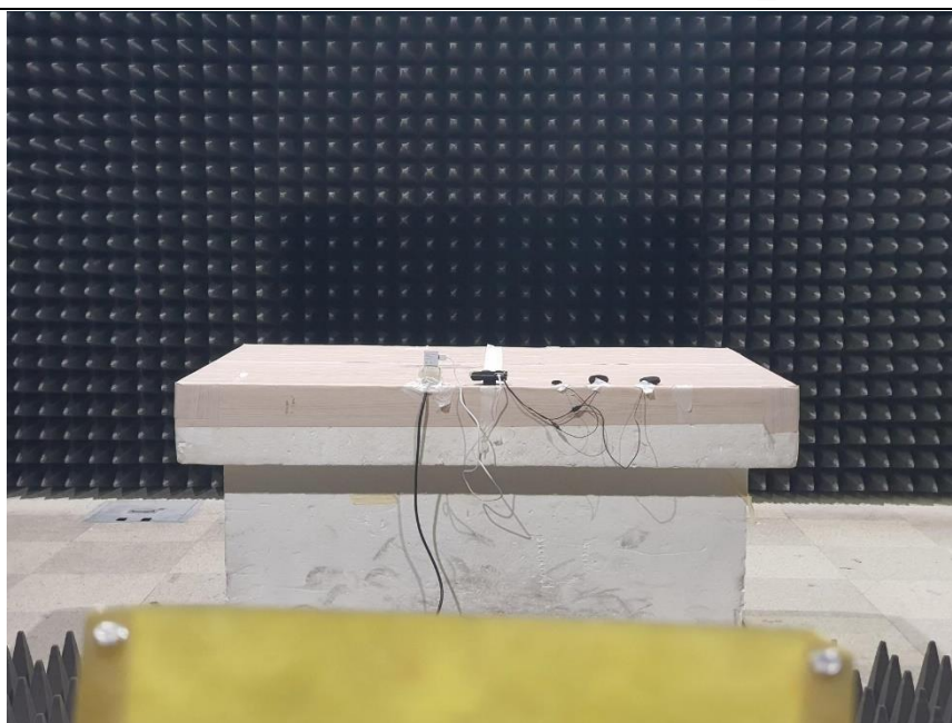
[Radiated Emission (3 m method Above 1GHz)_Rear]
