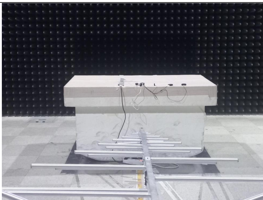
[Radiated Emission (3 m method Below 1GHz)_Rear]
