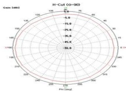
XY plane @2442MHz
