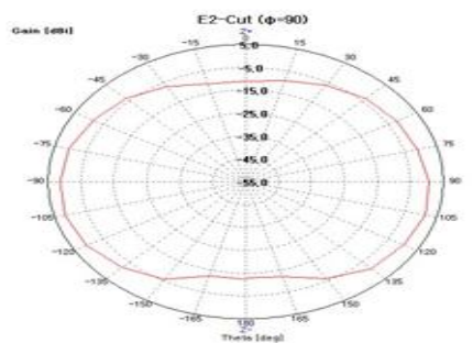
YZ plane @2442MHz
