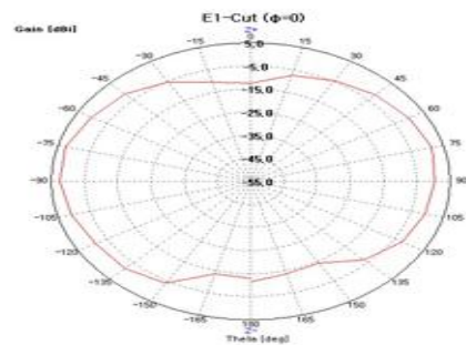
XZ plane @2442MHz
