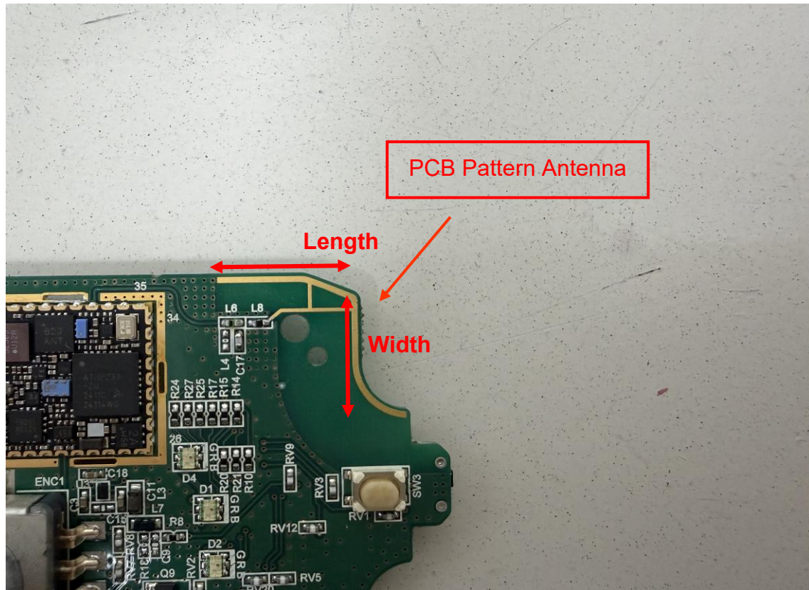
Internal PCB Pattern Antenna
