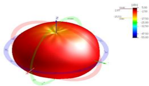
3D radiation pattern @2442MHz
