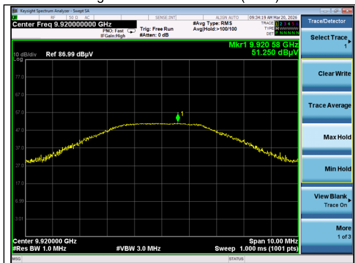
High channel 4 th harmonic (Peak)
