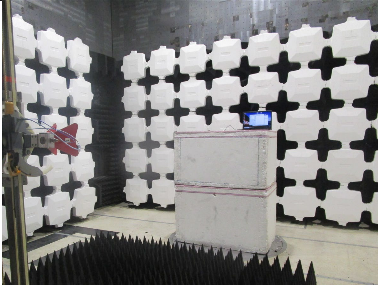
Radiated Testing, Above 1 GHz #2
