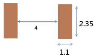
FootPrint (Unit : mm)
