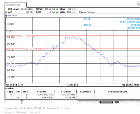
GFSK_Mid_DH1
