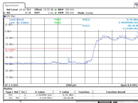
8DPSK_Hopping_Lower_3DH1
