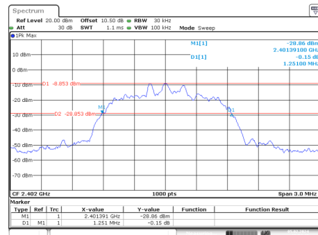
8DPSK_Low_3DH1
