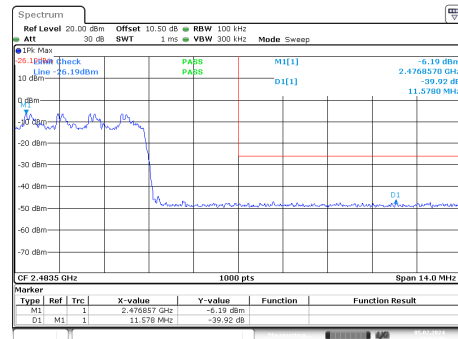
PI/4-DQPSK_Hopping_Upper_2DH1
