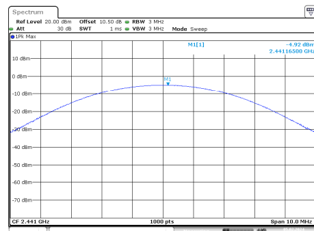
PI/4-DQPSK_Mid_2DH1
