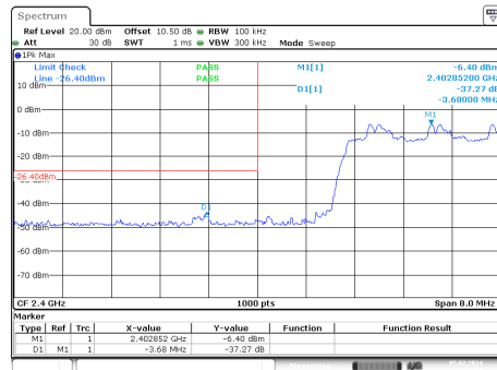
PI/4-DQPSK_Hopping_Lower_2DH1
