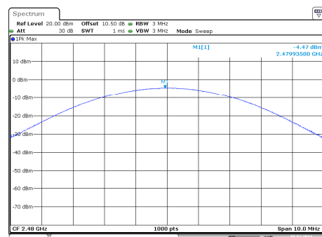
8DPSK_High_3DH1
