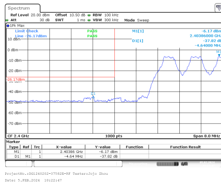
GFSK_Hopping_Lower_DH1
