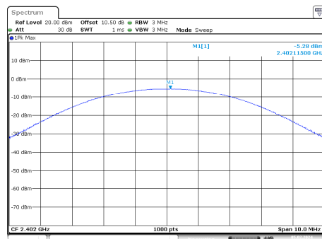
PI/4-DQPSK_Low_2DH1
