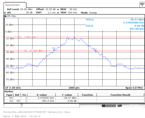
GFSK_High_DH1
