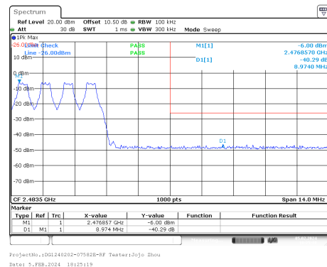
GFSK_Hopping_Upper_DH1
