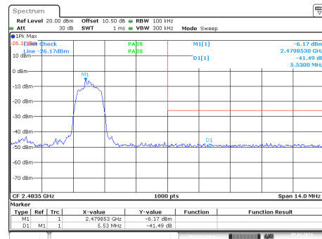
PI/4-DQPSK_High_2DH1
