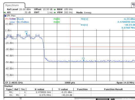
8DPSK_Hopping_Upper_3DH1
