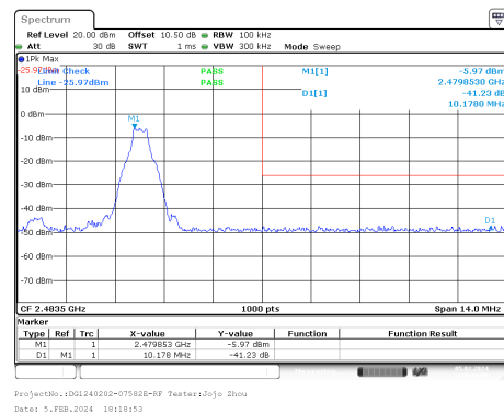
GFSK_High_DH1
