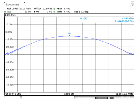
GFSK_Mid_DH1
