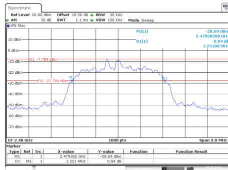
PI/4-DQPSK_High_2DH1
