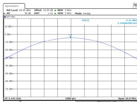
8DPSK_Mid_3DH1
