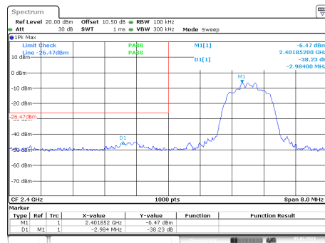
8DPSK_Low_3DH1
