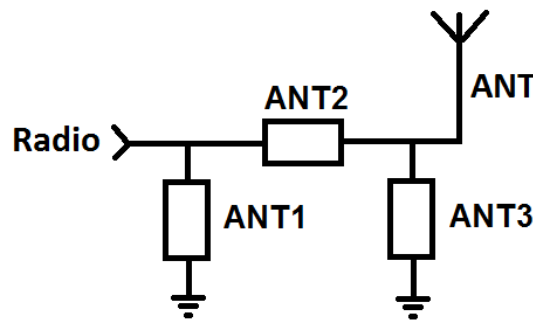
Figure 4. Antenna Match Network
