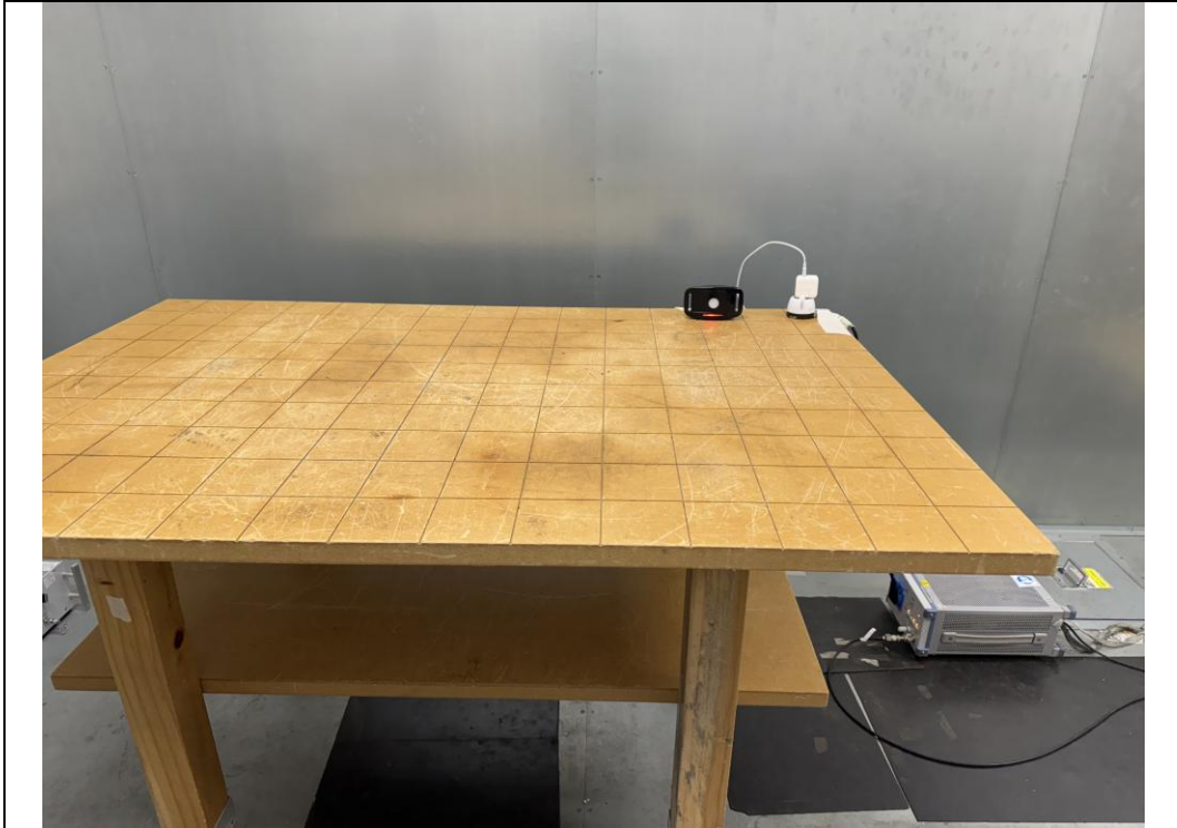
Conducted Emission_Front
