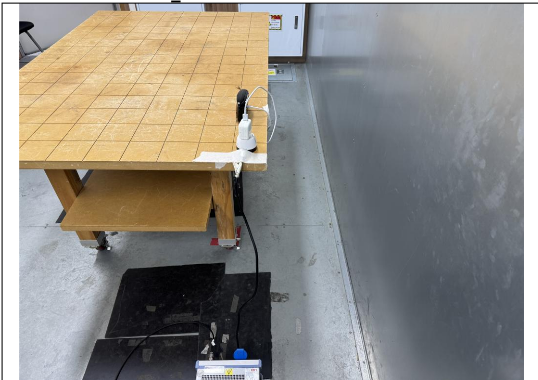
Conducted Emission_Rear
