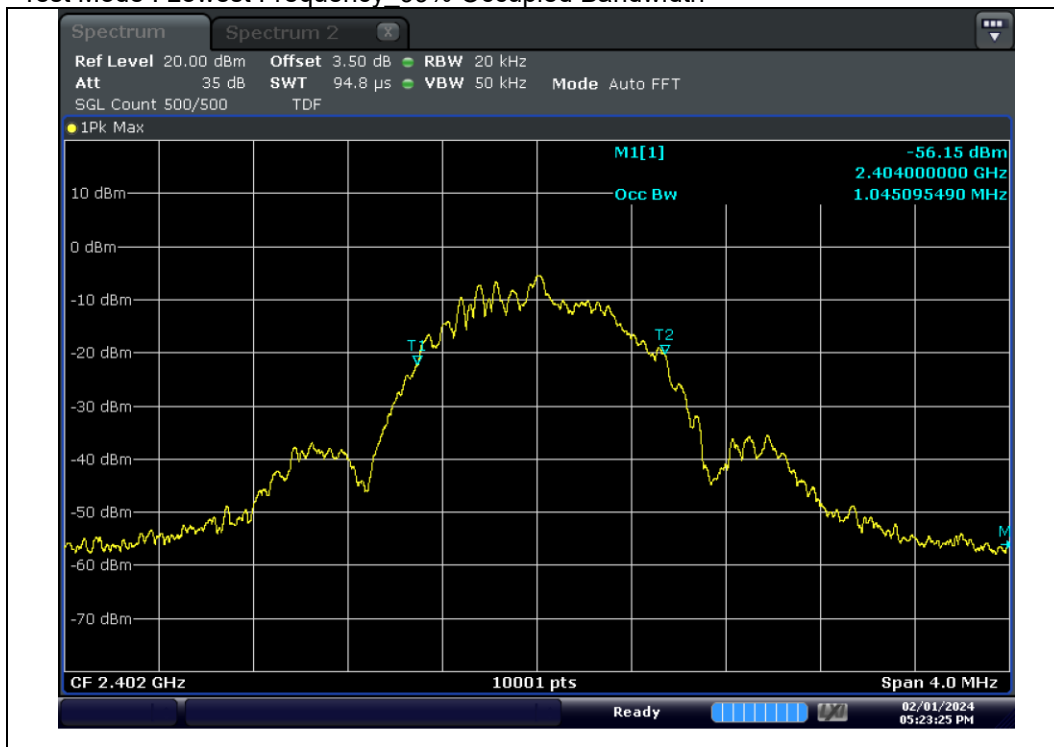
Test Mode : Lowest Frequency 99% Occupied Bandwidth
