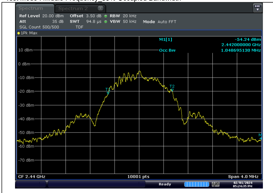
Test Mode : Middle Frequency 99% Occupied Bandwidth
