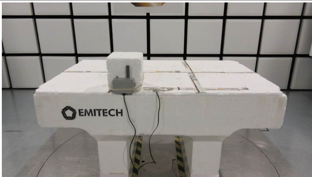
TEST SETUP PHOTO(S) - RADIATED MEASUREMENT / POSITION
