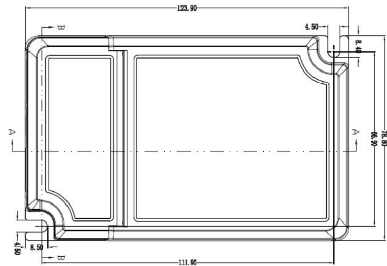
Figure 5: Mechanical Drawing
