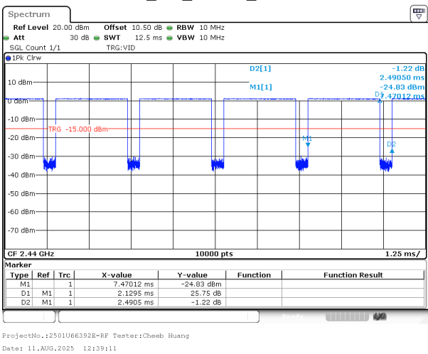
BLE_1M_Middle_Channel
