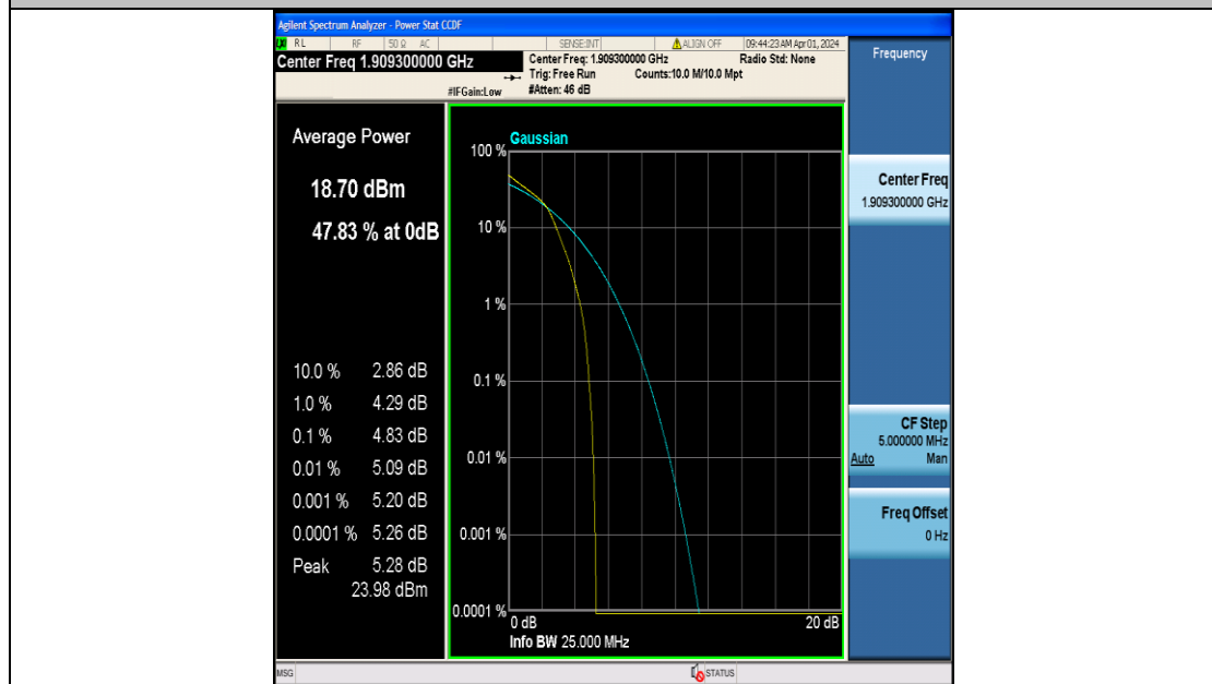
Band2-1.4MHz-16QAM-19193-6RB#0-PASS
