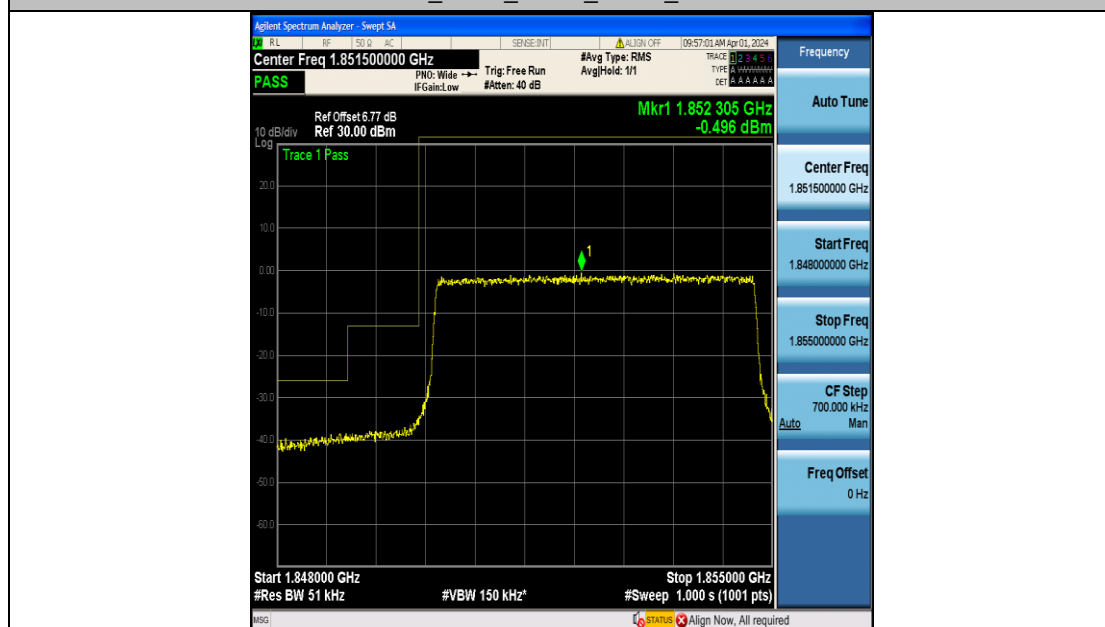
Band2_5MHz_16QAM_18625_25RB#0
