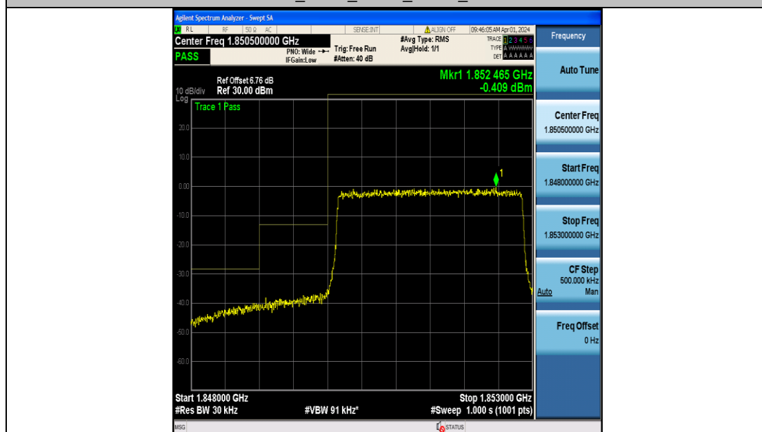
Band2_3MHz_16QAM_18615_15RB#0
