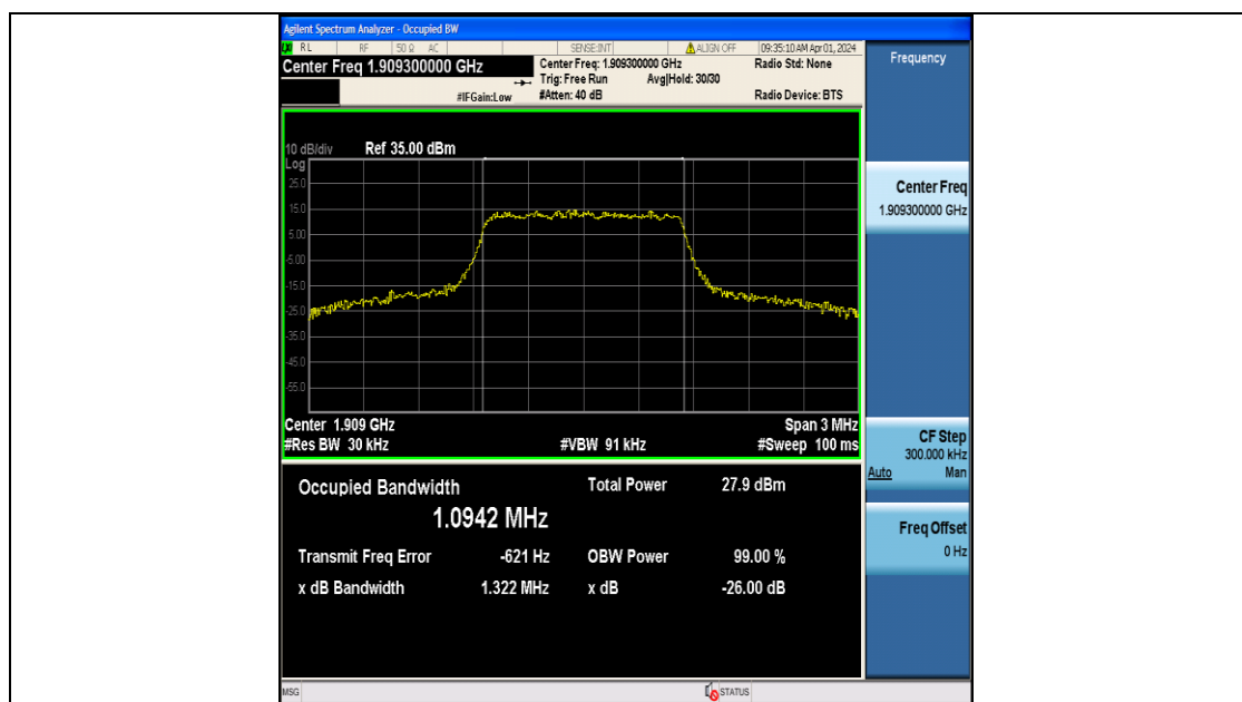
Band2-1.4MHz-QPSK-19193-6RB#0-PASS
