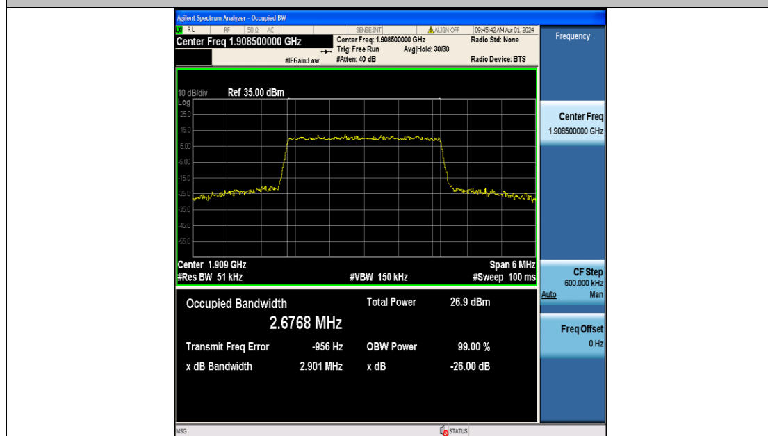
Band2-3MHz-16QAM-19185-15RB#0-PASS
