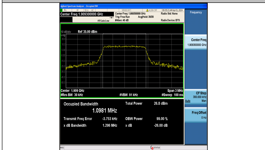
Band2-1.4MHz-16QAM-19193-6RB#0-PASS
