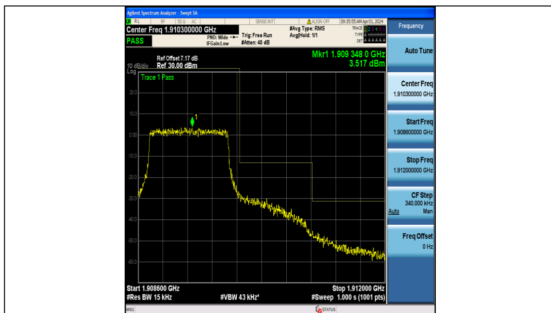
Band2_1.4MHz_QPSK_19193_6RB#0
