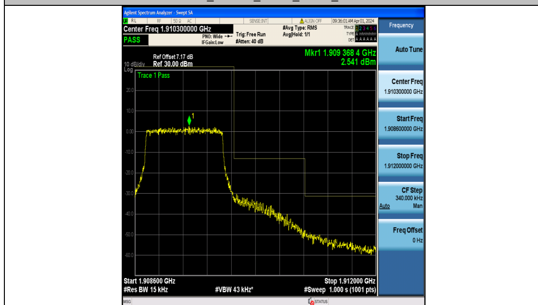
Band2_1.4MHz_16QAM_19193_6RB#0
