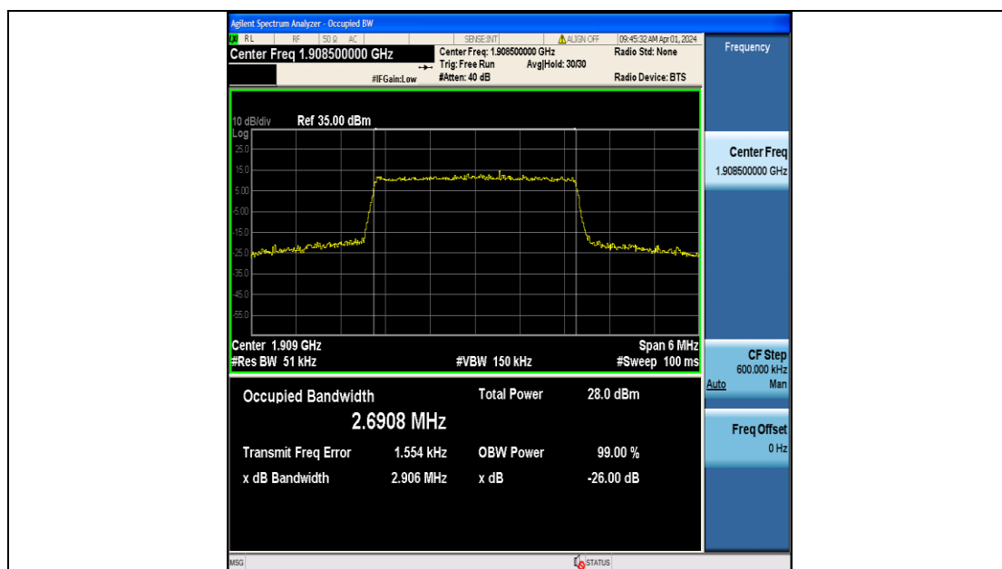
Band2-3MHz-QPSK-19185-15RB#0-PASS
