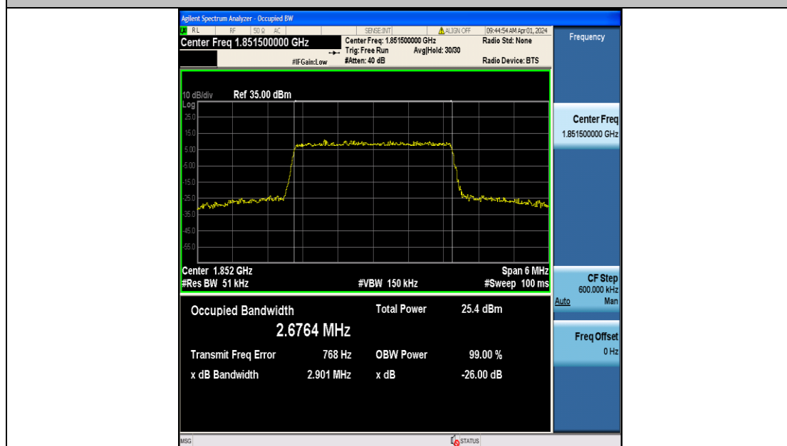
Band2-3MHz-16QAM-18615-15RB#0-PASS
