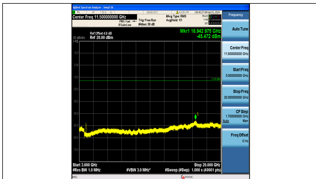
Band2_1.4MHz_16QAM_19193_6RB#0_3000~20000_3000~20000
