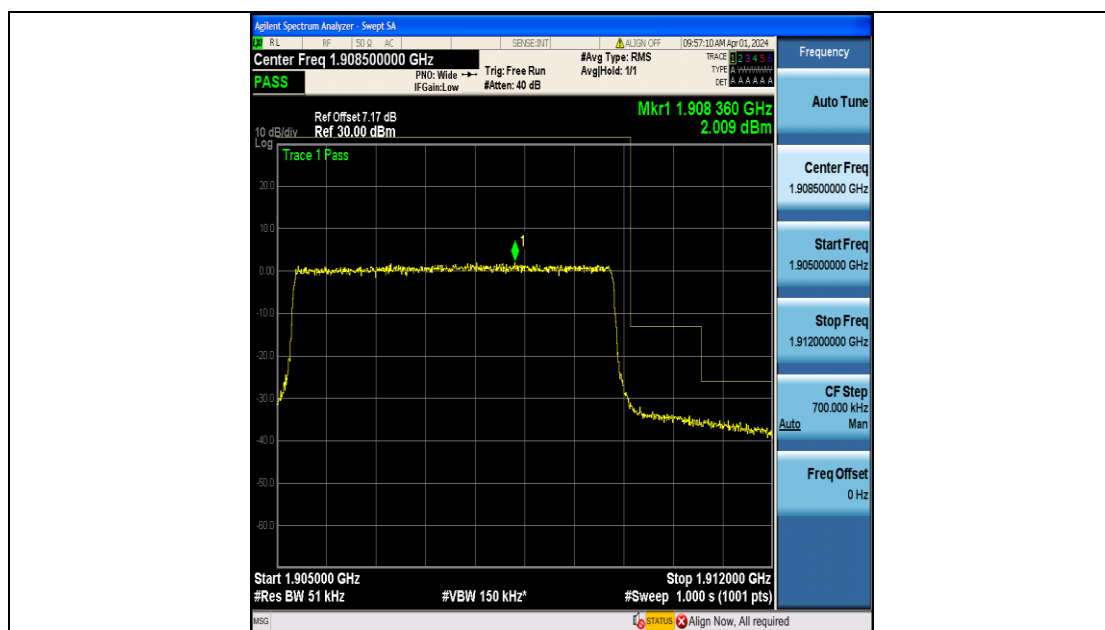
Band2_5MHz_QPSK_19175_25RB#0
