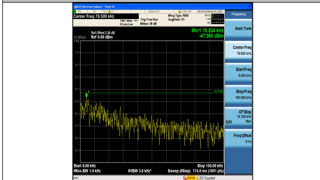
Band2_3MHz_QPSK_19185_15RB#0_0.009~0.15_0.009~0.15
