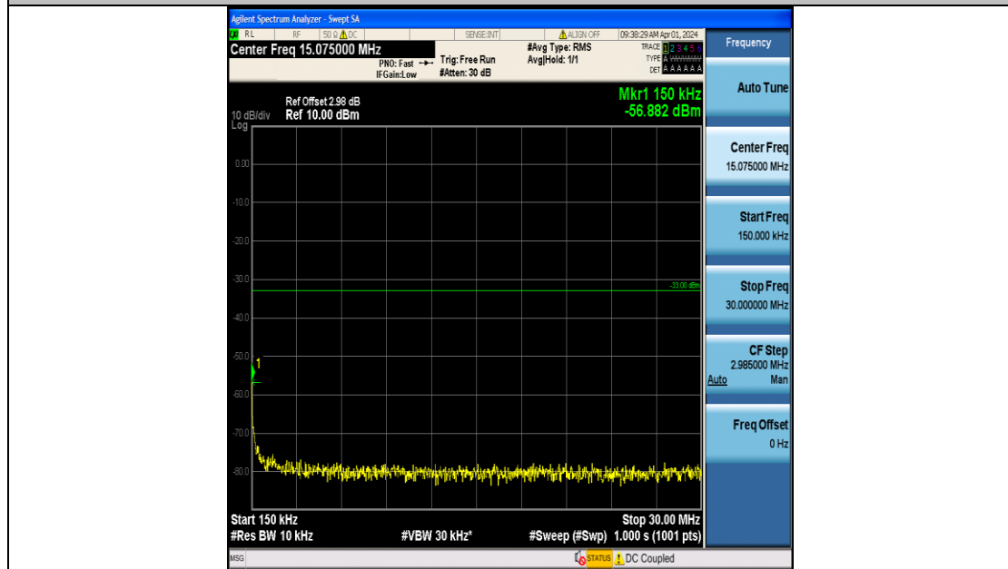
Band2_1.4MHz_16QAM_18900_6RB#0_0.15~30_0.15~30
