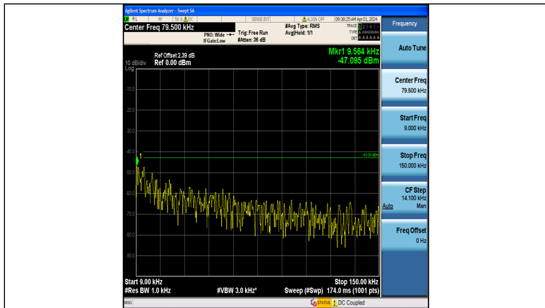
Band2_1.4MHz_16QAM_18900_6RB#0_0.009~0.15_0.009~0.15
