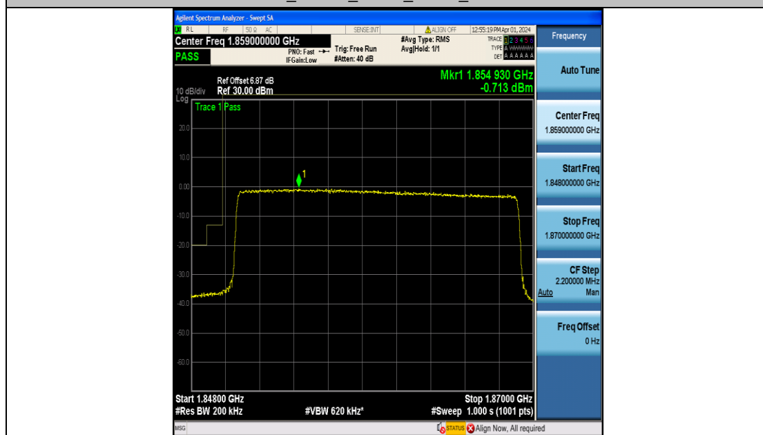
Band2_20MHz_16QAM_18700_100RB#0
