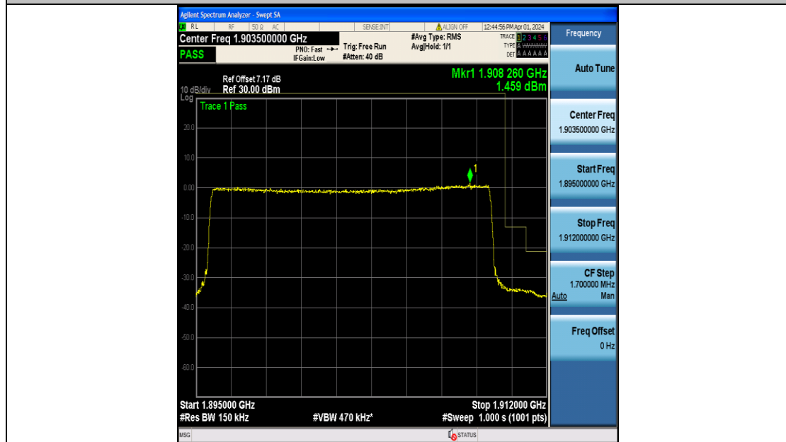
Band2_15MHz_16QAM_19125_75RB#0
