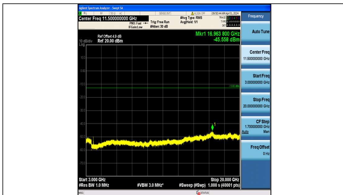
Band2_3MHz_16QAM_19185_15RB#0_3000~20000_3000~20000
