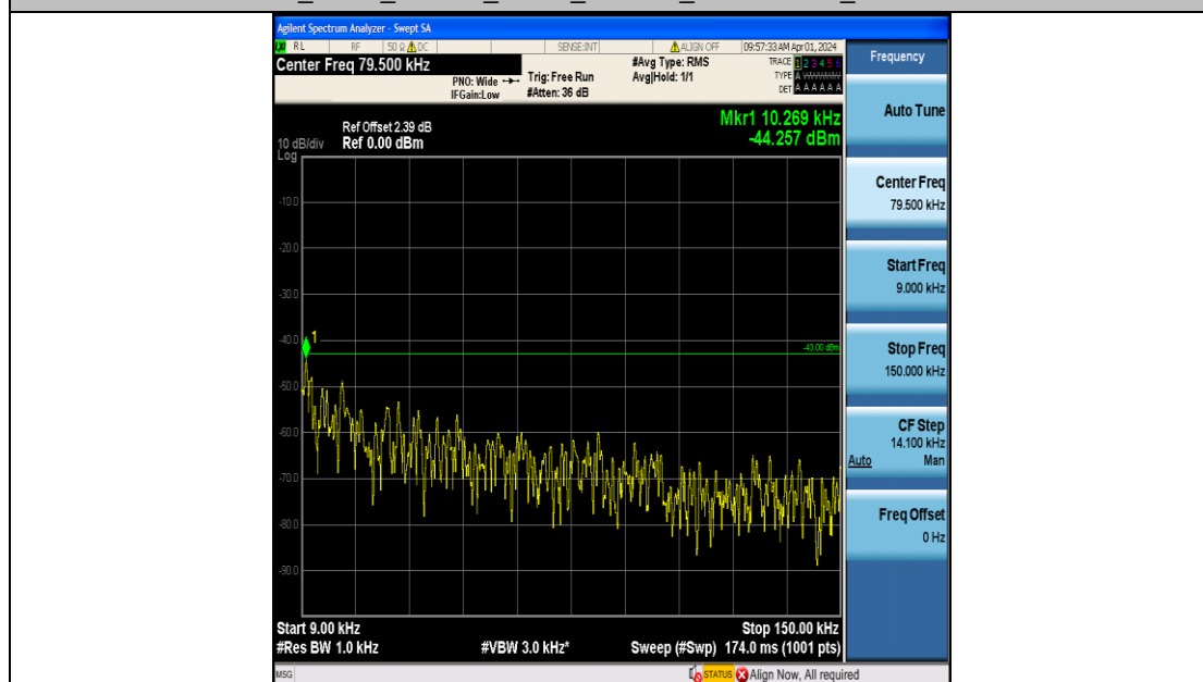
Band2_5MHz_QPSK_18625_25RB#0_0.009~0.15_0.009~0.15
