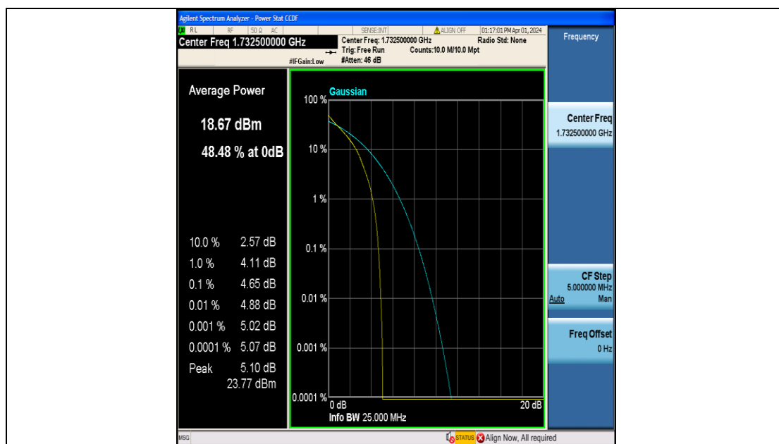
Band4-1.4MHz-QPSK-20175-6RB#0-PASS
