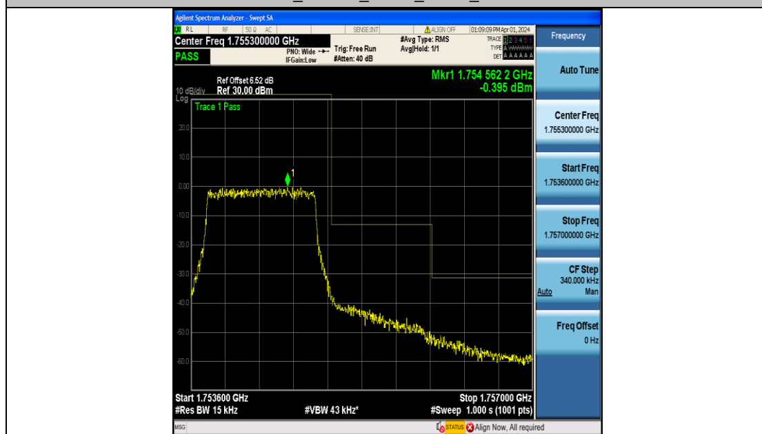
Band4_1.4MHz_16QAM_20393_6RB#0
