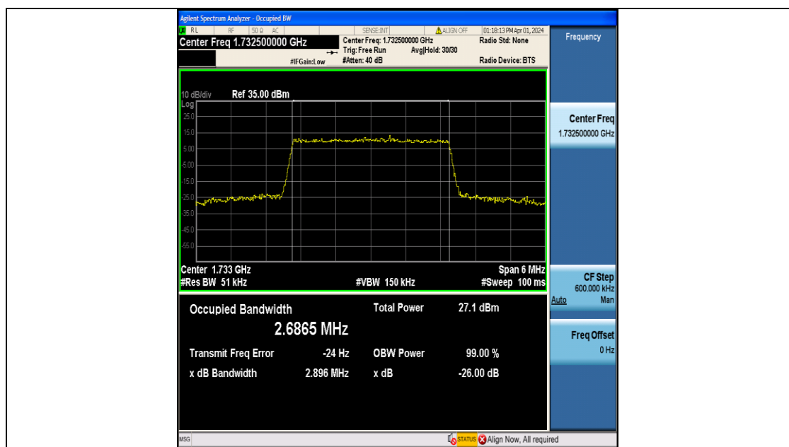
Band4-3MHz-QPSK-20175-15RB#0-PASS
