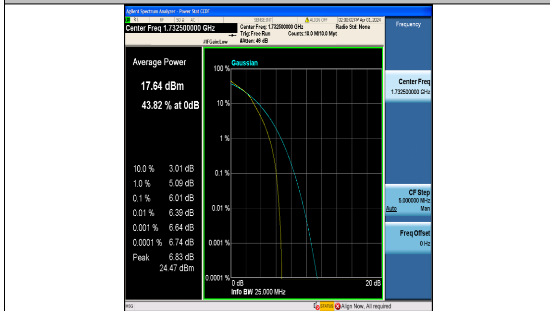
Band4-15MHz-16QAM-20175-75RB#0-PASS
