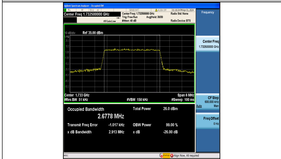
Band4-3MHz-16QAM-20175-15RB#0-PASS
