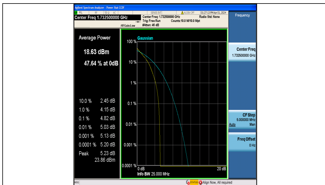
Band4-3MHz-QPSK-20175-15RB#0-PASS
