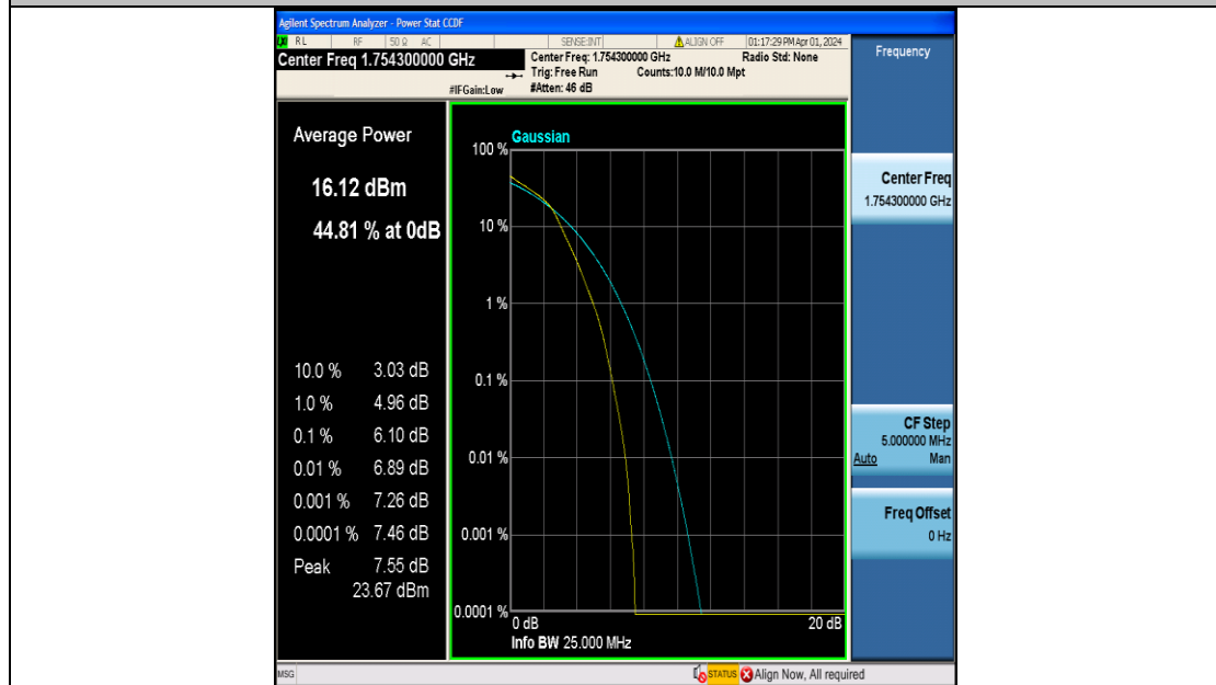
Band4-1.4MHz-16QAM-20393-6RB#0-PASS
