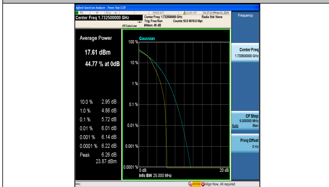
Band4-3MHz-16QAM-20175-15RB#0-PASS
