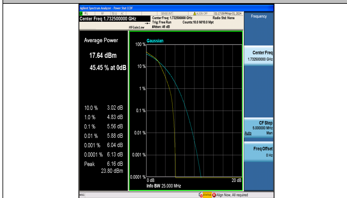
Band4-1.4MHz-16QAM-20175-6RB#0-PASS
