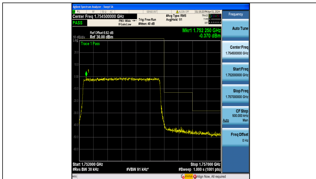
Band4_3MHz_QPSK_20385_15RB#0
