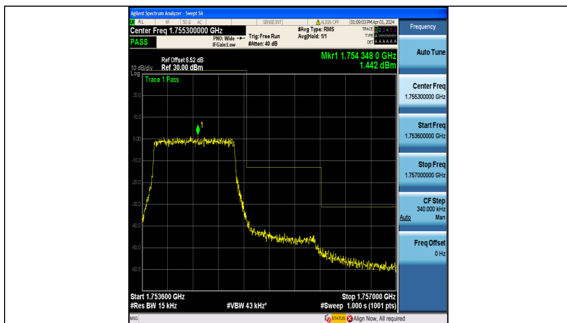
Band4_1.4MHz_QPSK_20393_6RB#0
