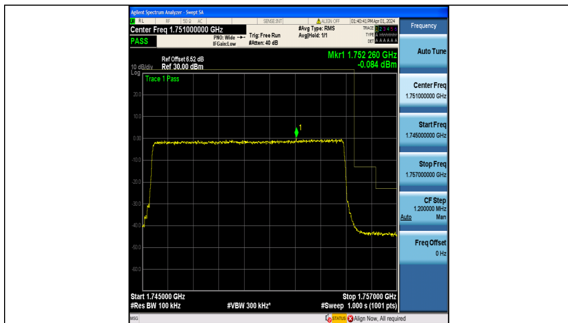
Band4_10MHz_QPSK_20350_50RB#0
