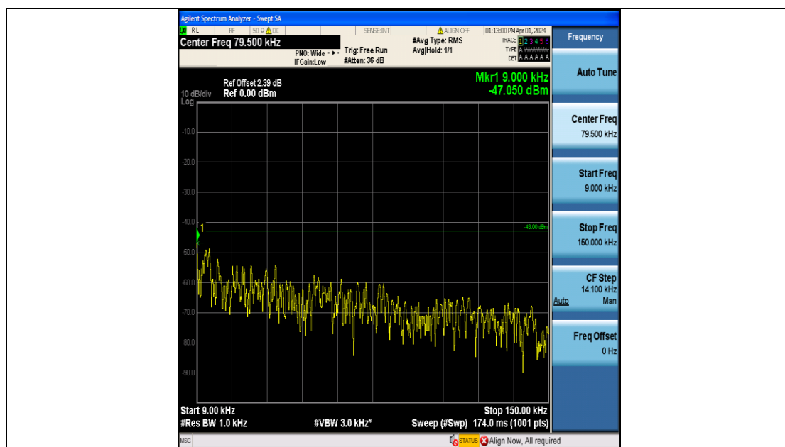
Band4_1.4MHz_16QAM_20393_6RB#0_0.009~0.15_0.009~0.15
