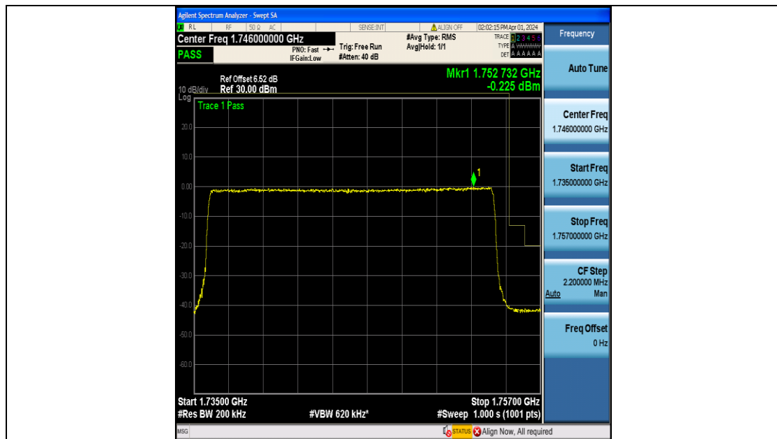
Band4_20MHz_QPSK_20300_100RB#0
