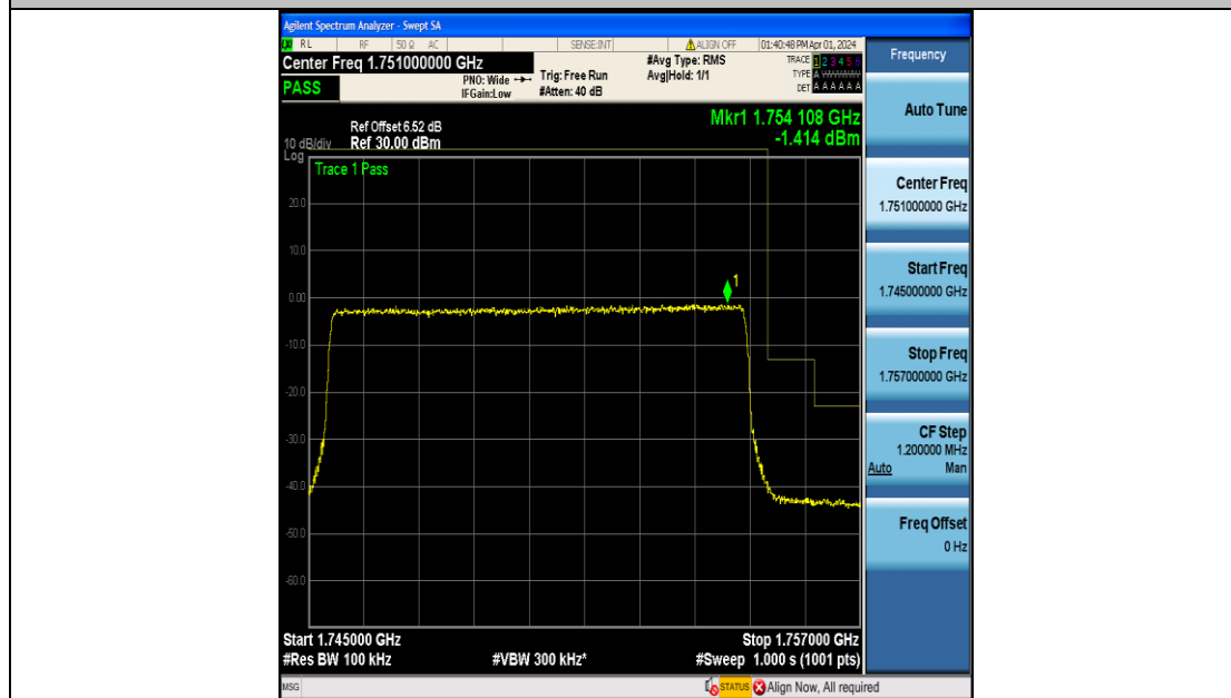
Band4_10MHz_16QAM_20350_50RB#0
