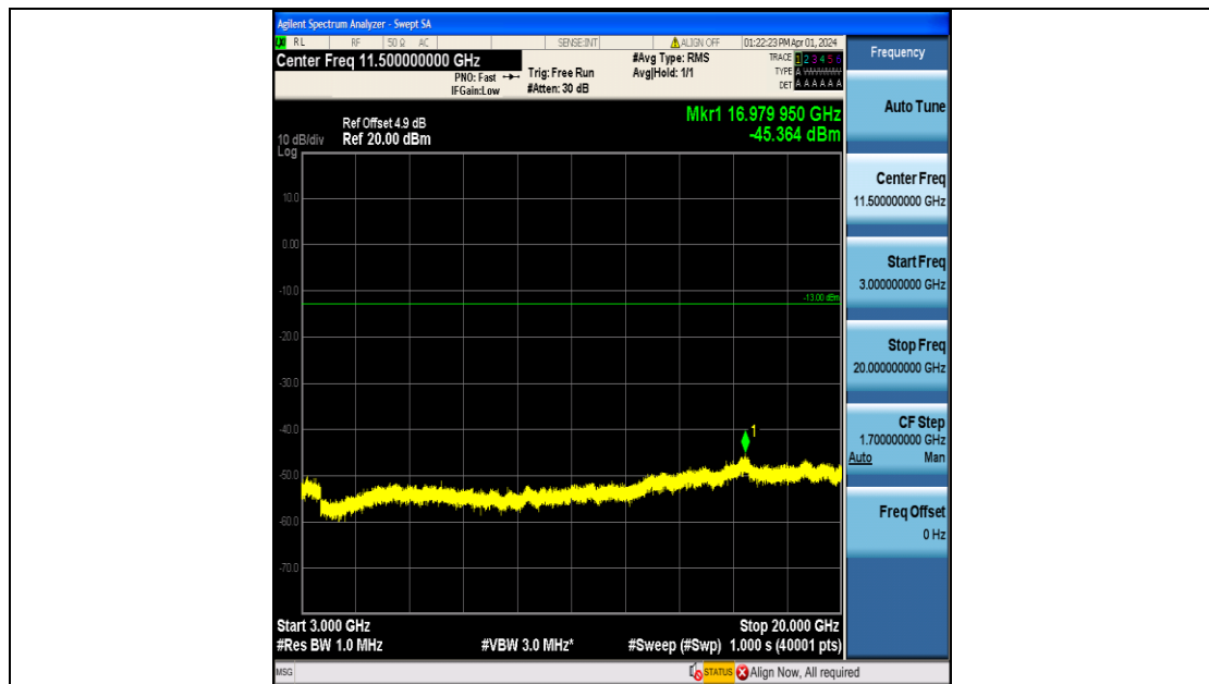
Band4_3MHz_16QAM_20175_15RB#0_3000~20000_3000~20000
