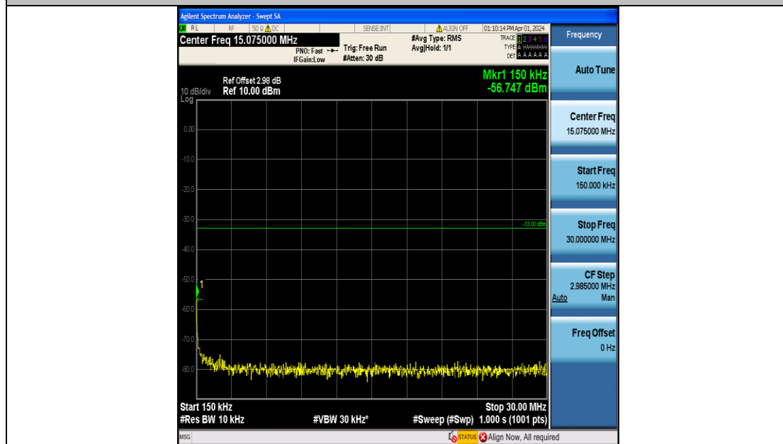
Band4_1.4MHz_16QAM_19957_6RB#0_0.15~30_0.15~30
