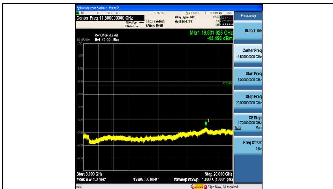
Band4_1.4MHz_16QAM_20393_6RB#0_3000~20000_3000~20000
