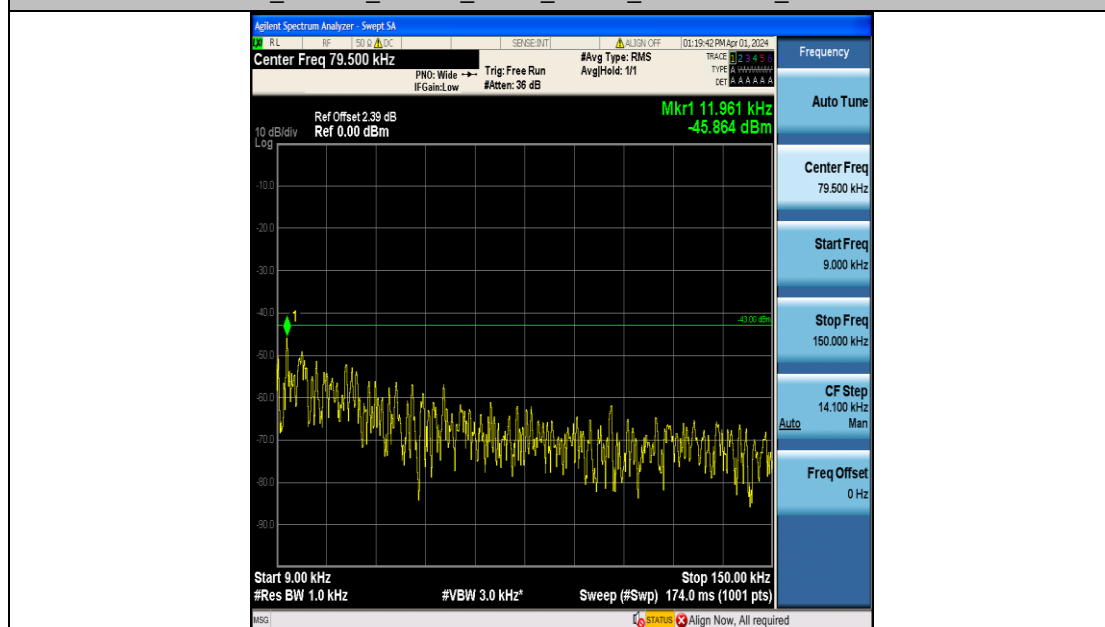
Band4_3MHz_QPSK_19965_15RB#0_0.009~0.15_0.009~0.15
