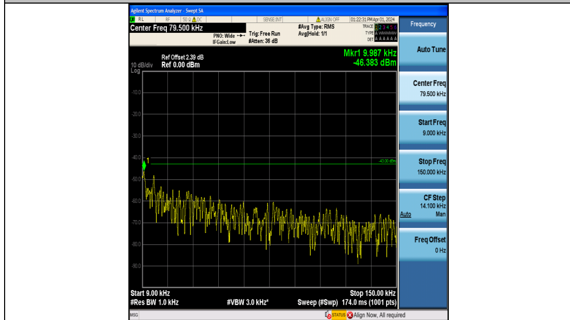
Band4_3MHz_QPSK_20385_15RB#0_0.009~0.15_0.009~0.15
