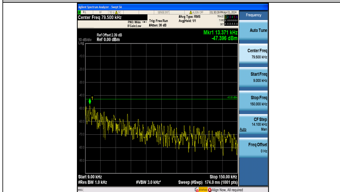
Band4_5MHz_QPSK_19975_25RB#0_0.009~0.15_0.009~0.15
