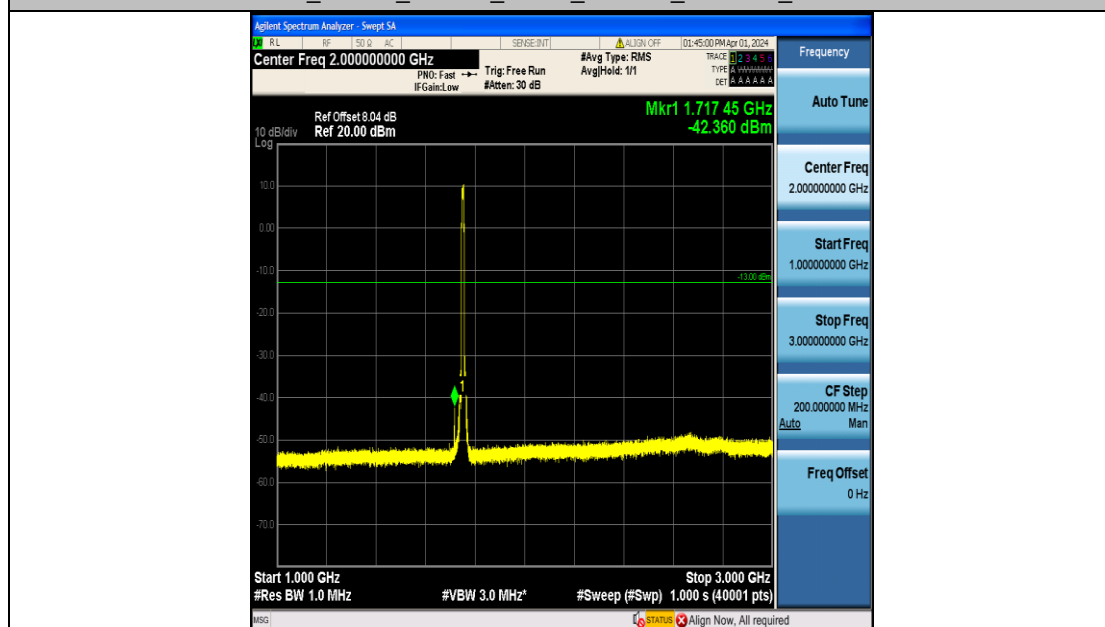
Band4_10MHz_16QAM_20350_50RB#0_1000~3000_1000~3000
