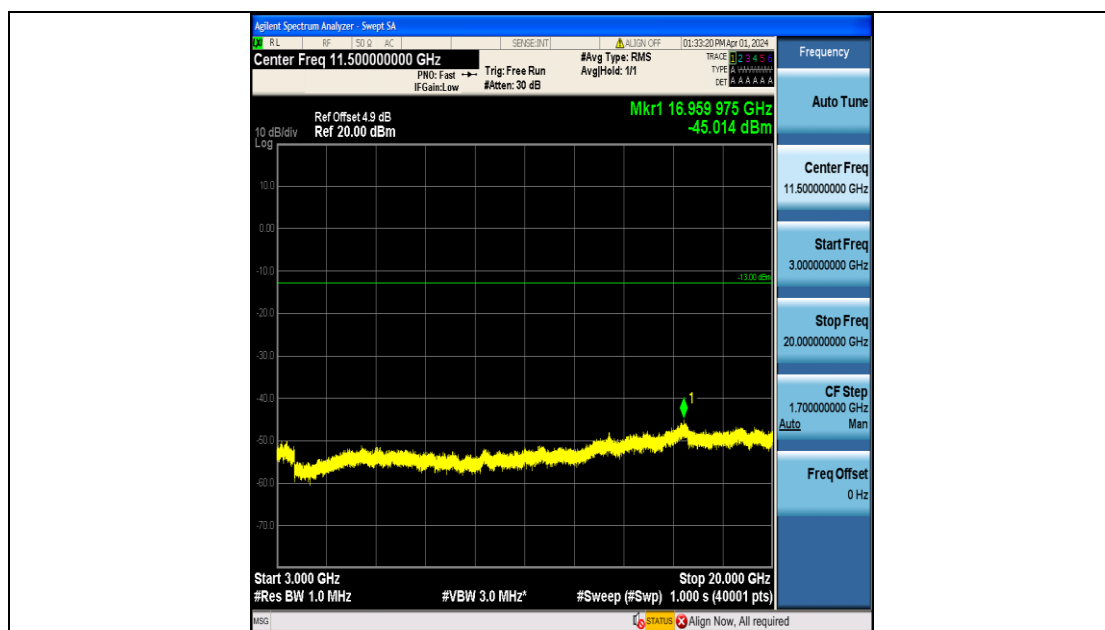
Band4_5MHz_16QAM_20175_25RB#0_3000~20000_3000~20000
