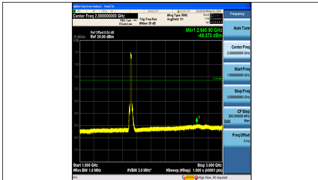
Band4_20MHz_QPSK_20050_100RB#0_1000~3000_1000~3000
