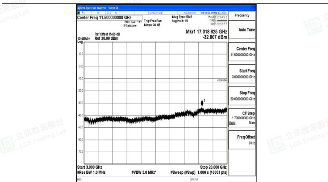
Band2_10MHz_QPSK_18650_1RB#0_3000~20000_3000~20000
