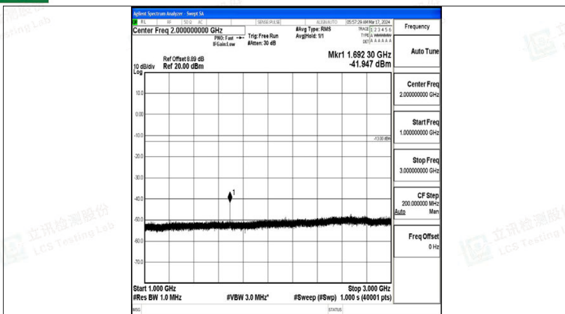
Band5_3MHz_16QAM_20635_1RB#0_1000~3000_1000~3000
