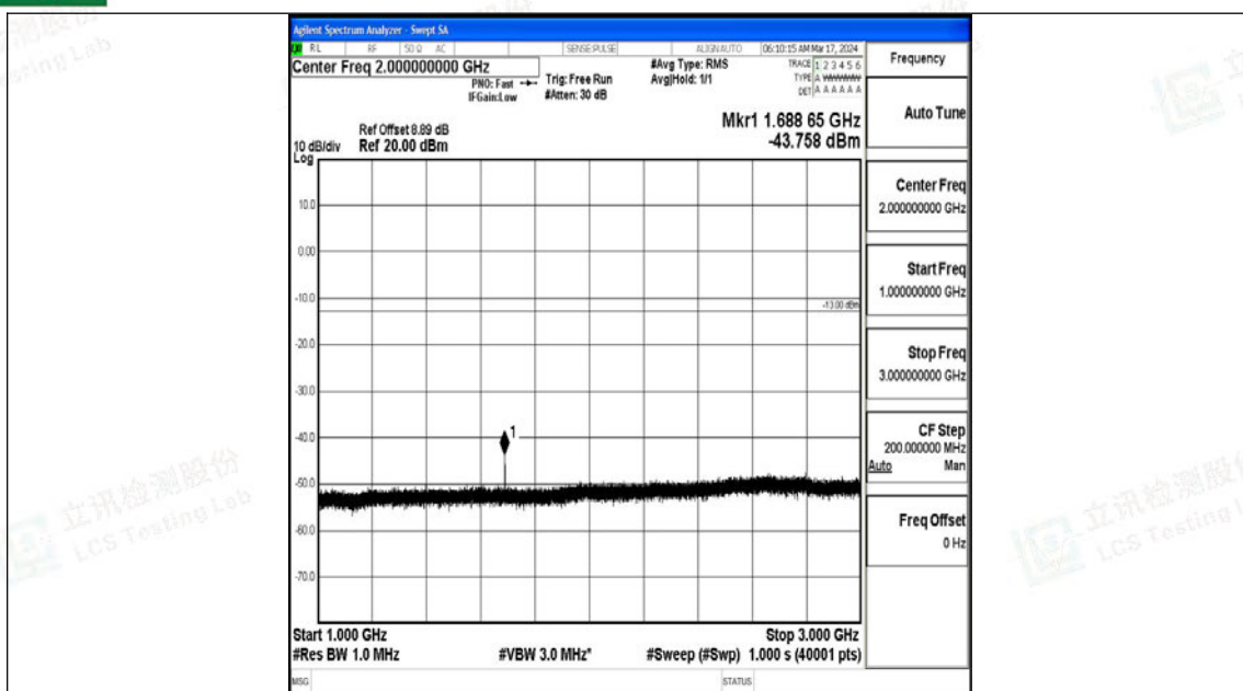
Band5_5MHz_16QAM_20625_1RB#0_1000~3000_1000~3000
