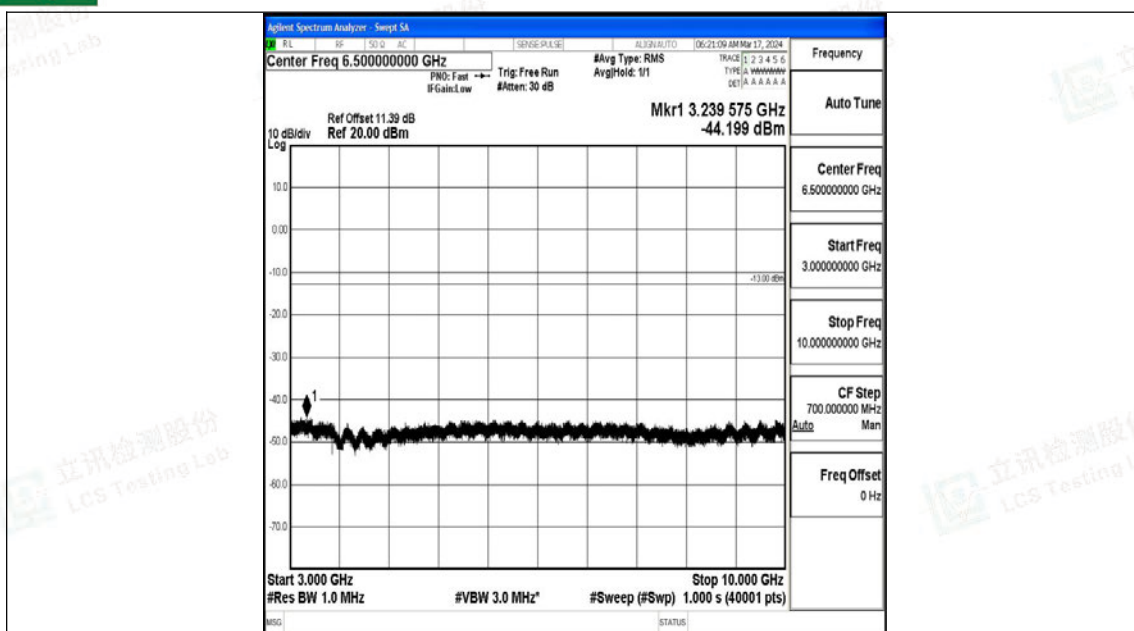
Band5_10MHz_QPSK_20525_1RB#0_3000~10000_3000~10000
