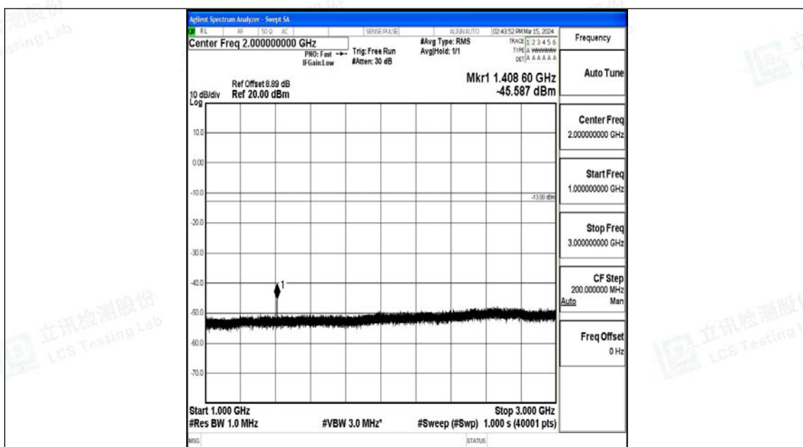
Band17_5MHz_16QAM_23755_1RB#0_1000~3000_1000~3000
