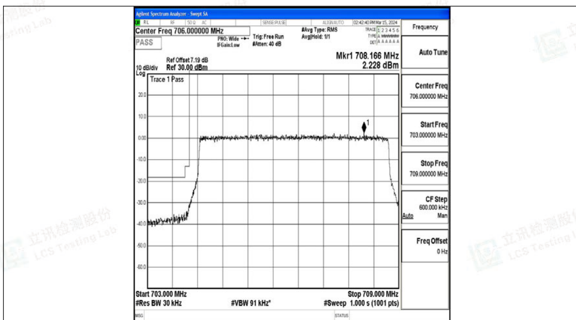
Band17_5MHz_16QAM_23755_25RB#0
