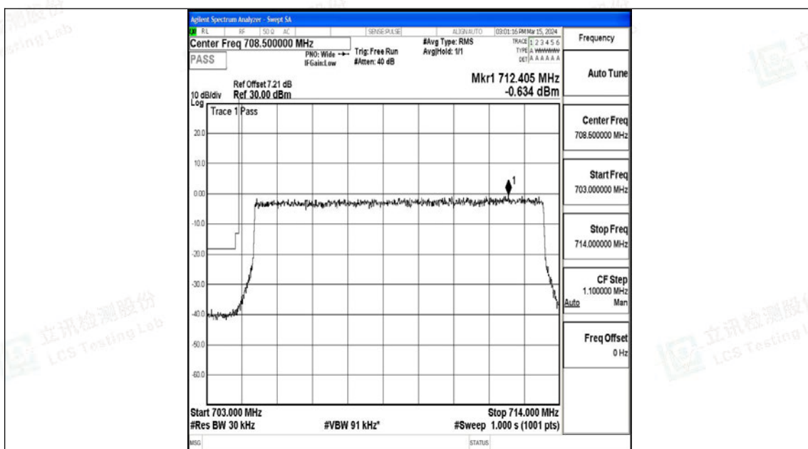
Band17_10MHz_16QAM_23780_50RB#0
