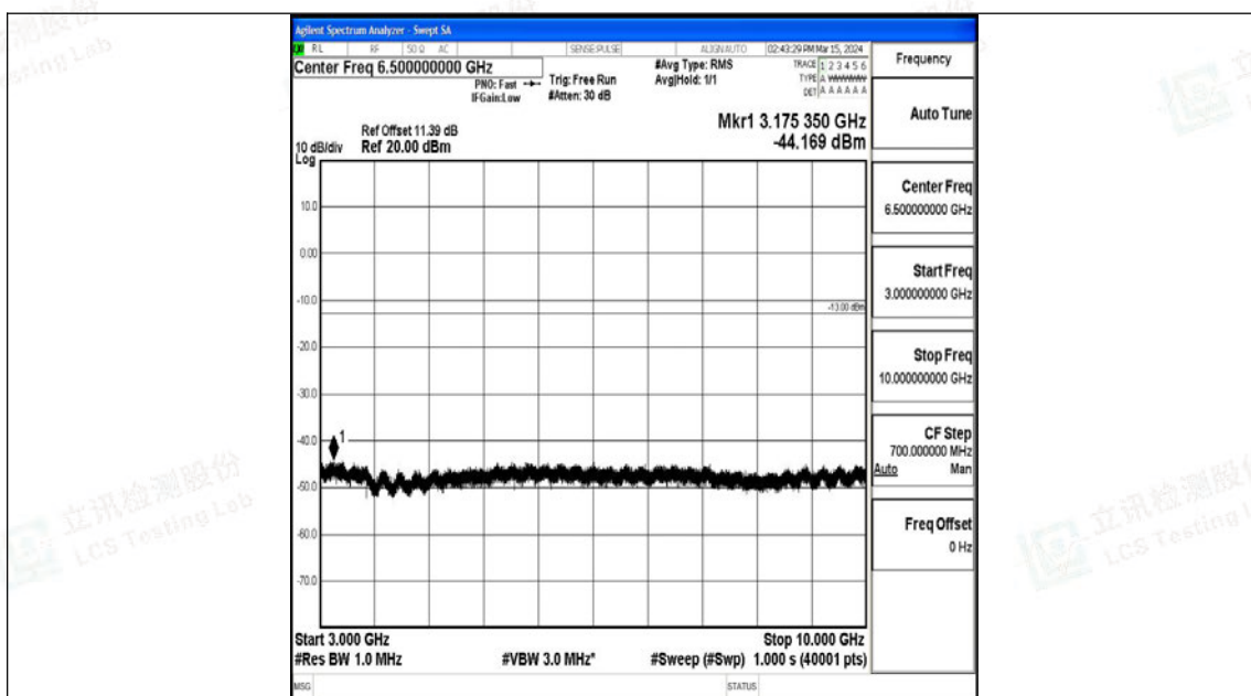
Band17_5MHz_QPSK_23755_1RB#0_3000~10000_3000~10000
