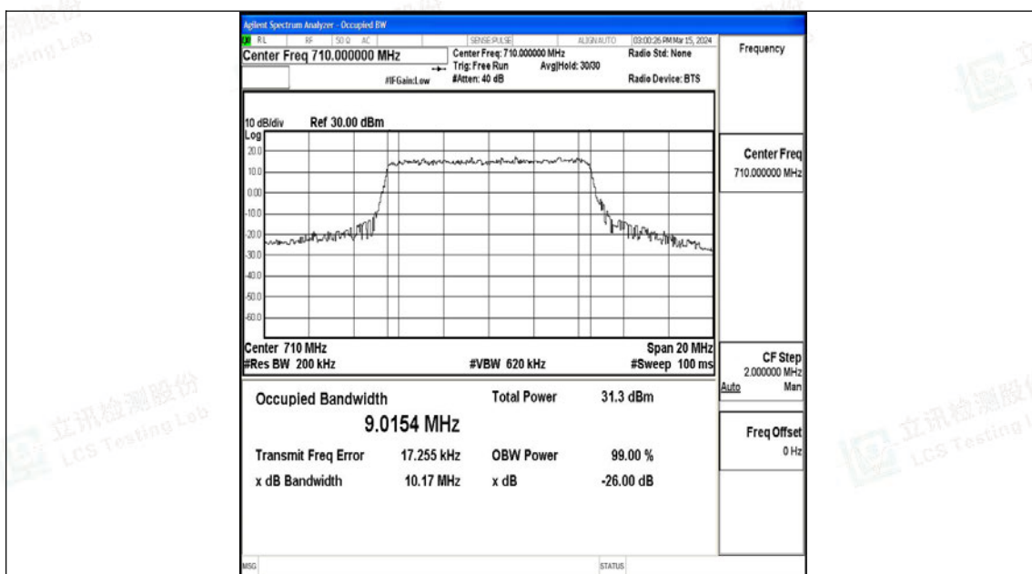
Band17-10MHz-QPSK-23790-50RB#0-PASS
