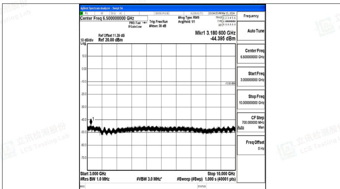
Band17_10MHz_QPSK_23800_1RB#0_3000~10000_3000~10000
