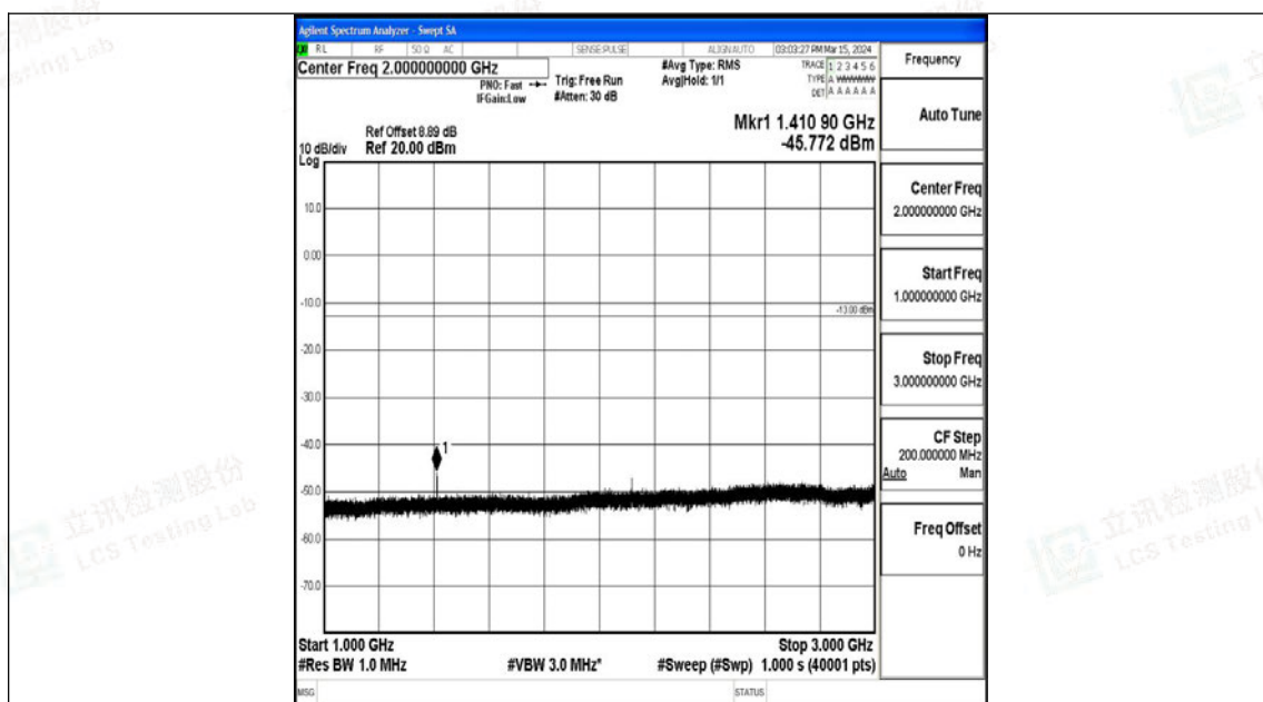
Band17_10MHz_16QAM_23790_1RB#0_1000~3000_1000~3000
