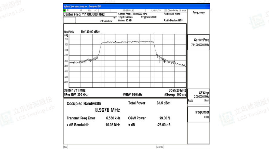
Band17-10MHz-QPSK-23800-50RB#0-PASS
