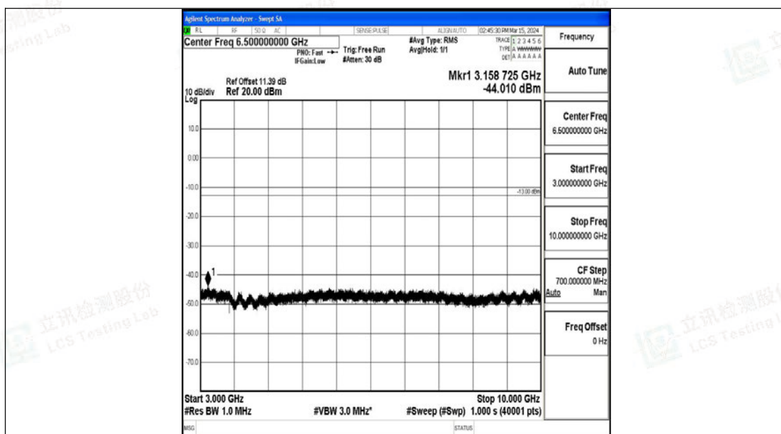
Band17_5MHz_QPSK_23825_1RB#0_3000~10000_3000~10000
