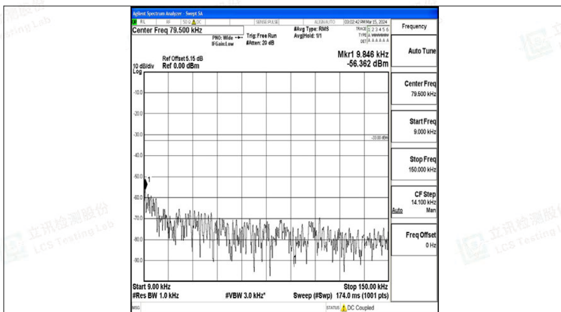
Band17_10MHz_QPSK_23790_1RB#0_0.009~0.15_0.009~0.15
