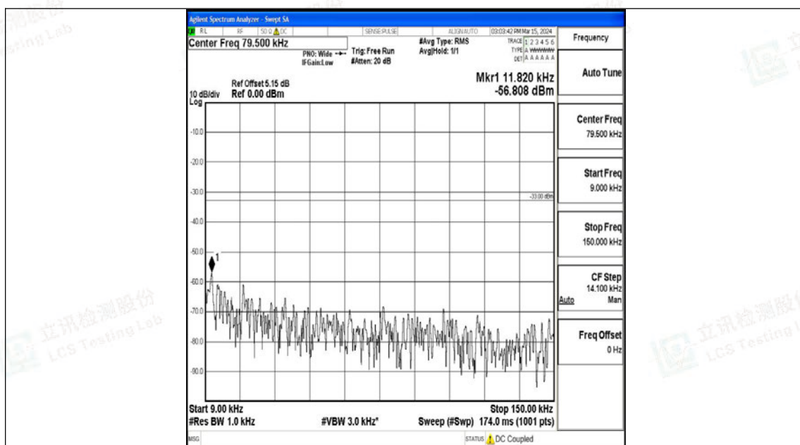
Band17_10MHz_QPSK_23800_1RB#0_0.009~0.15_0.009~0.15
