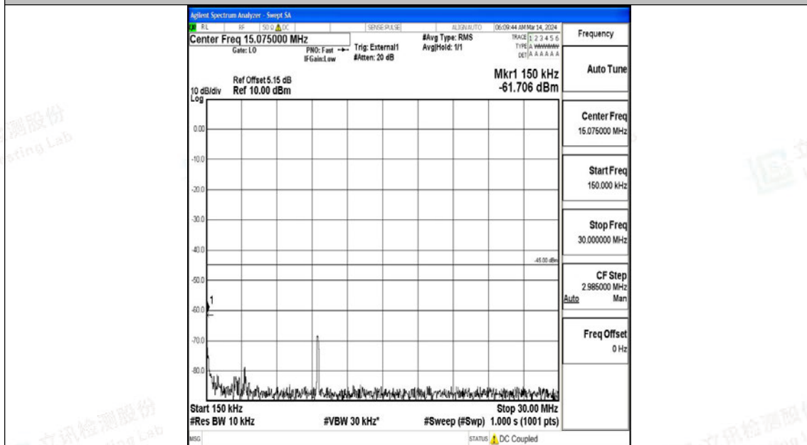
Band38_15MHz_QPSK_37825_1RB#0_0.15~30_0.15~30
