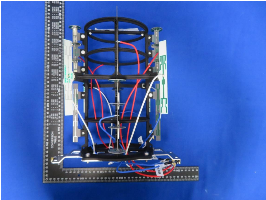
(11) EUT Photo-Omni Antenna
