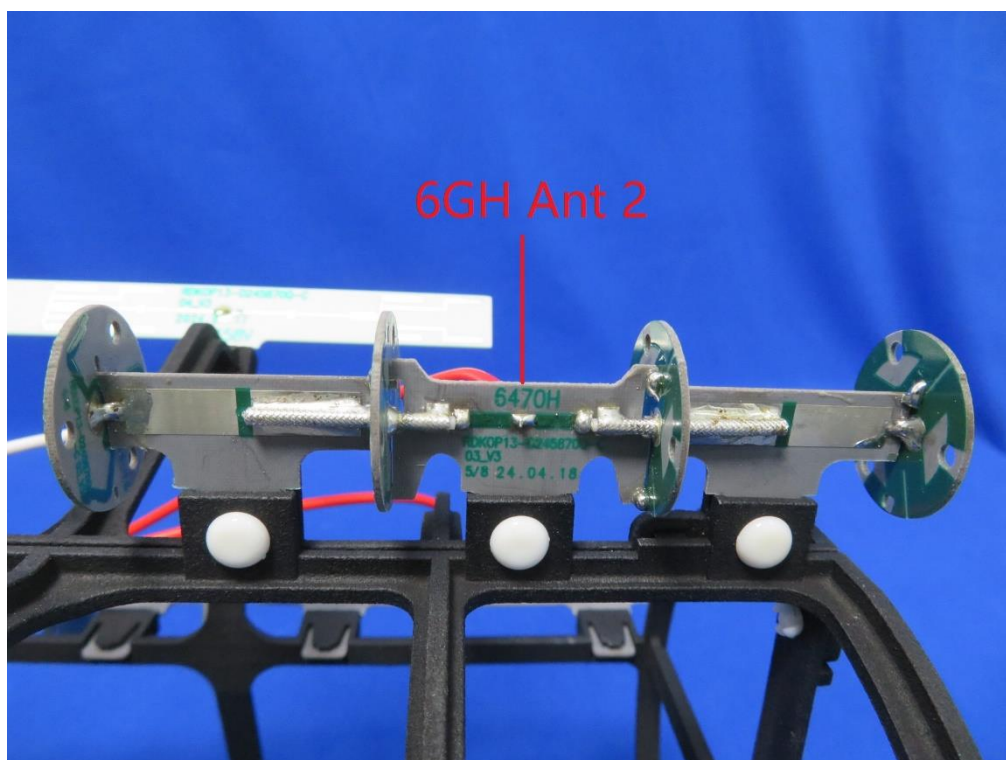
(18) EUT Photo-Omni Antenna
