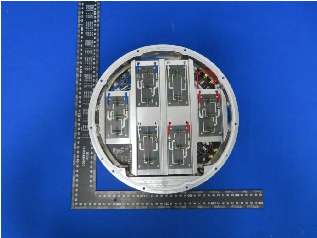
(26) EUT Photo-Directional Antenna
