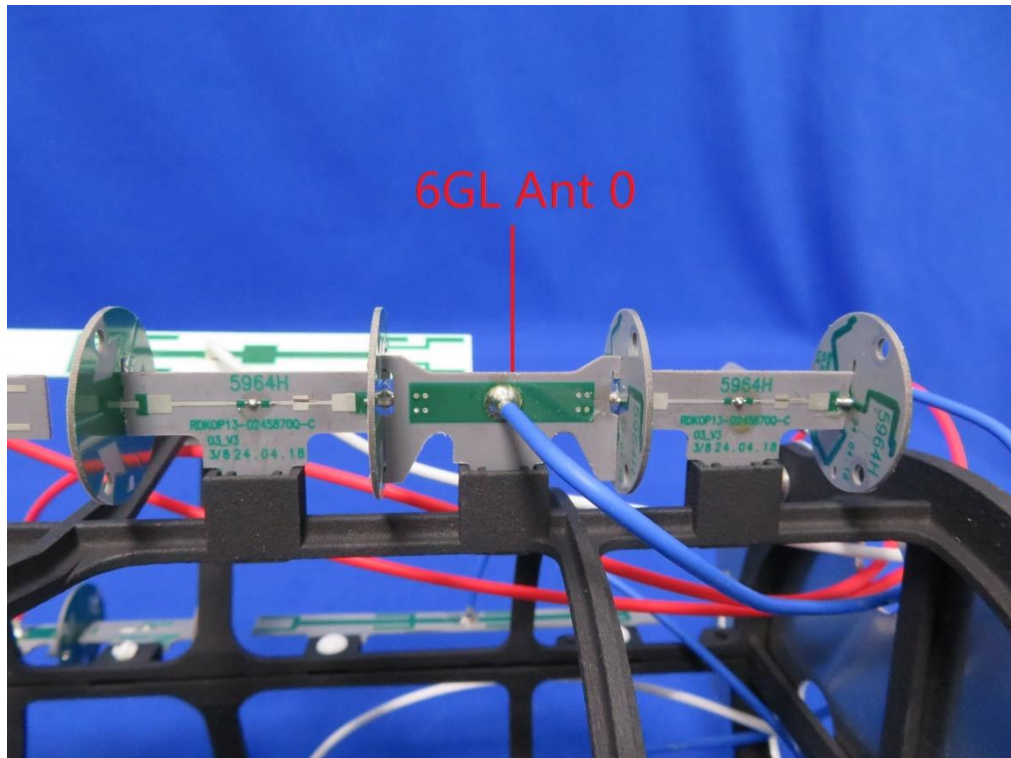
(21) EUT Photo-Omni Antenna
