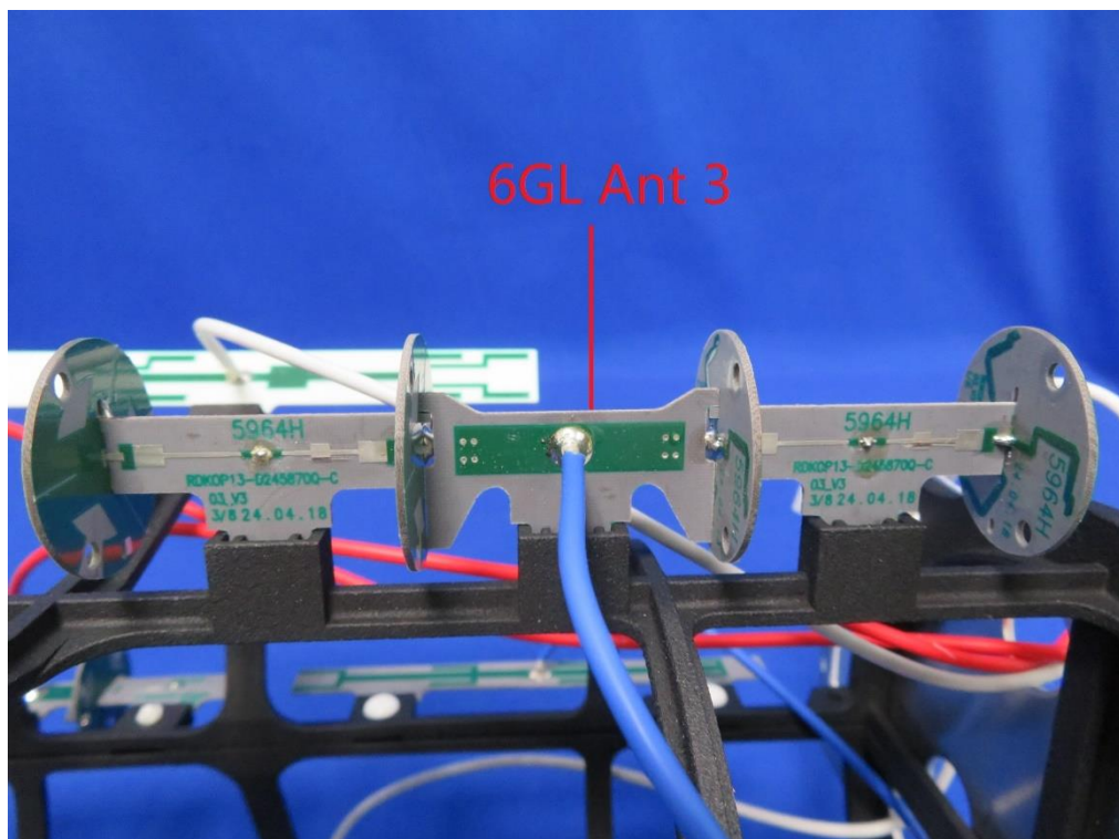
(24) EUT Photo-Omni Antenna
