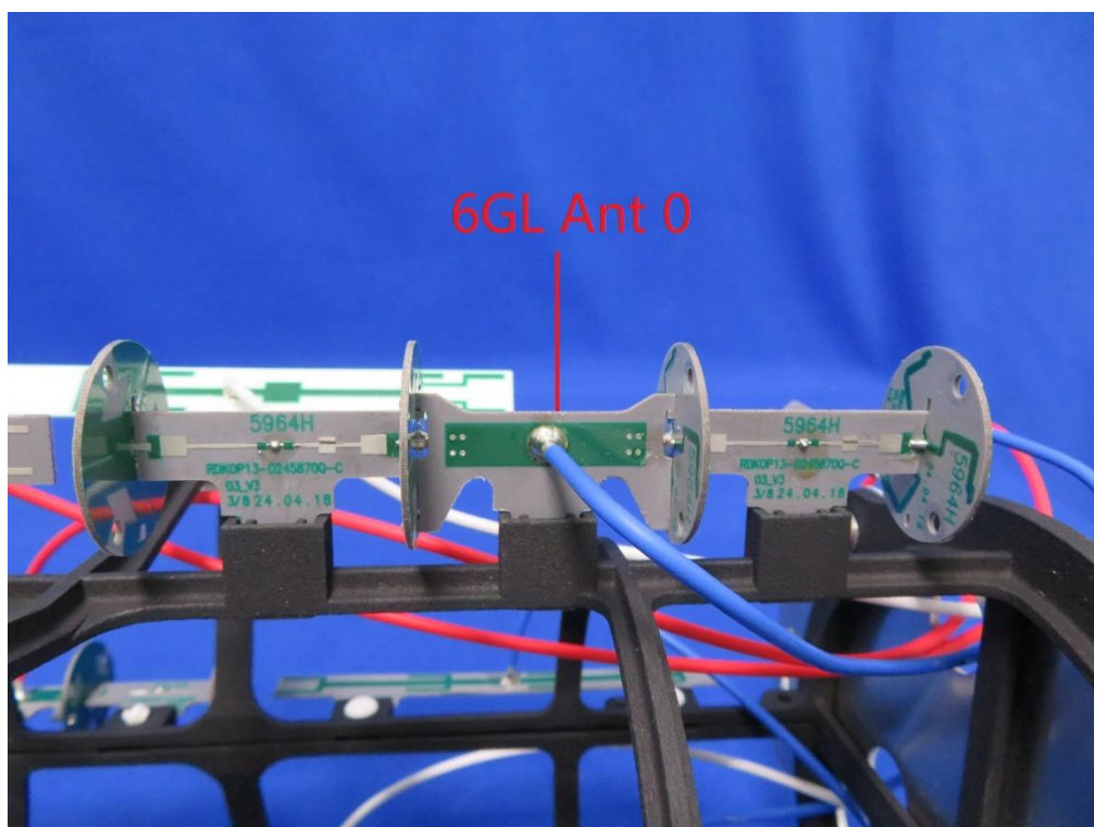
(20) EUT Photo-Omni Antenna
