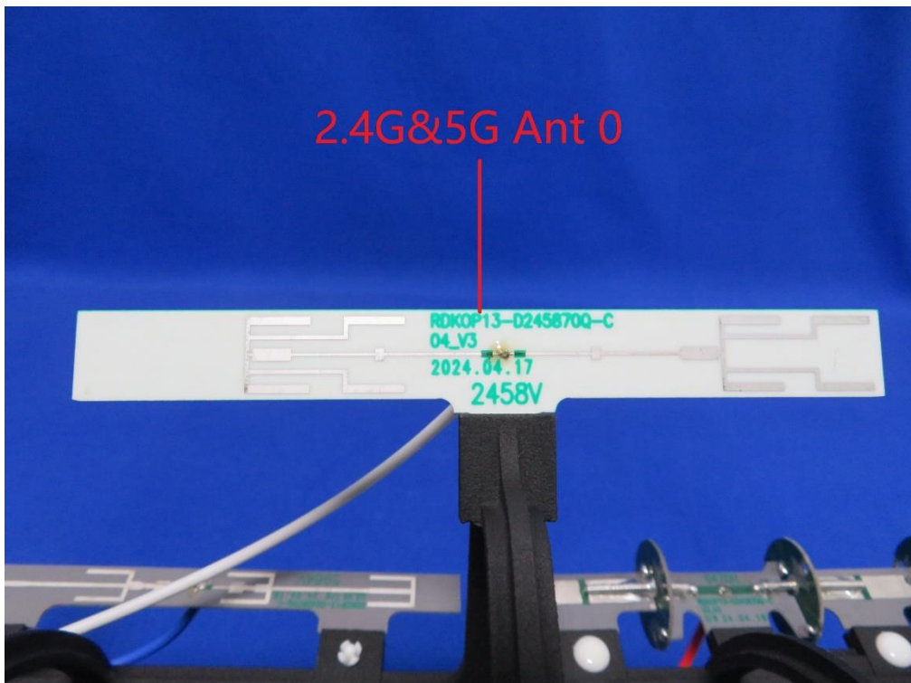
(12) EUT Photo-Omni Antenna
