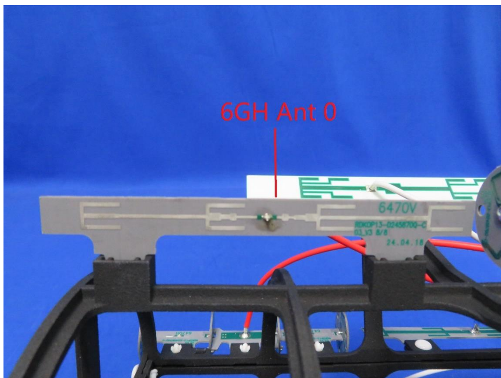
(17) EUT Photo-Omni Antenna
