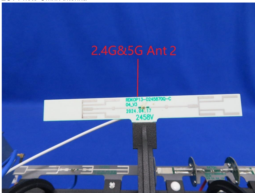
(14) EUT Photo-Omni Antenna
