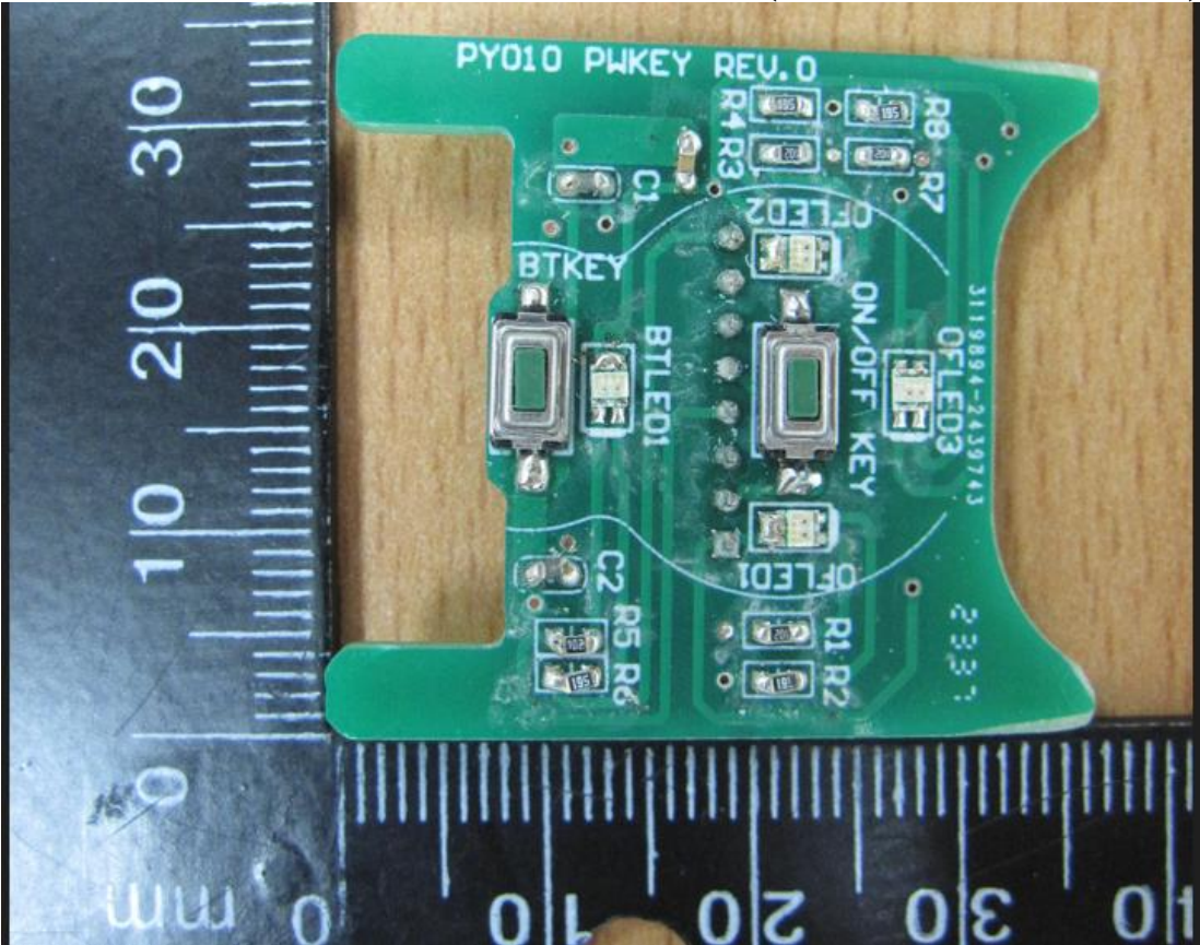
Figure 9 Internal View (Control Board, Front View)
