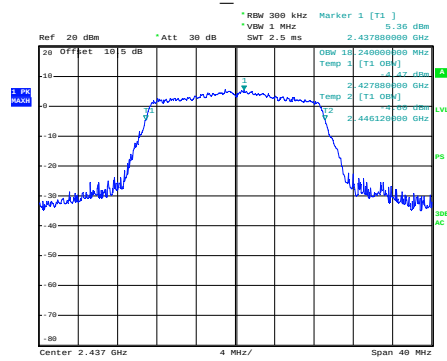
n20_2437MHz
