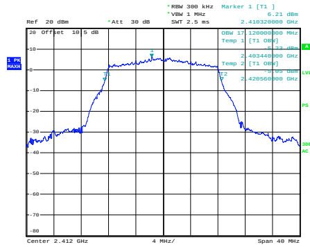
g_2412MHz
