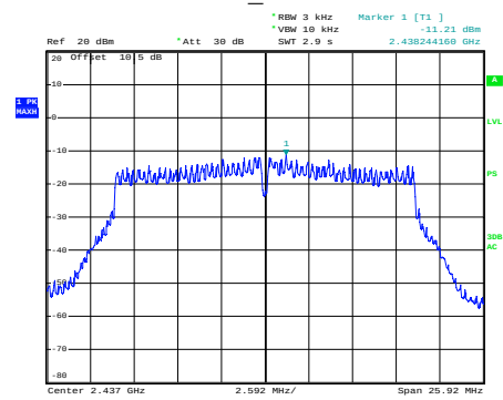
n20_2437MHz
