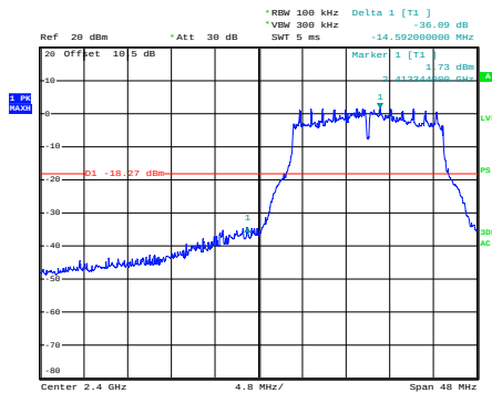
g_2412MHz
