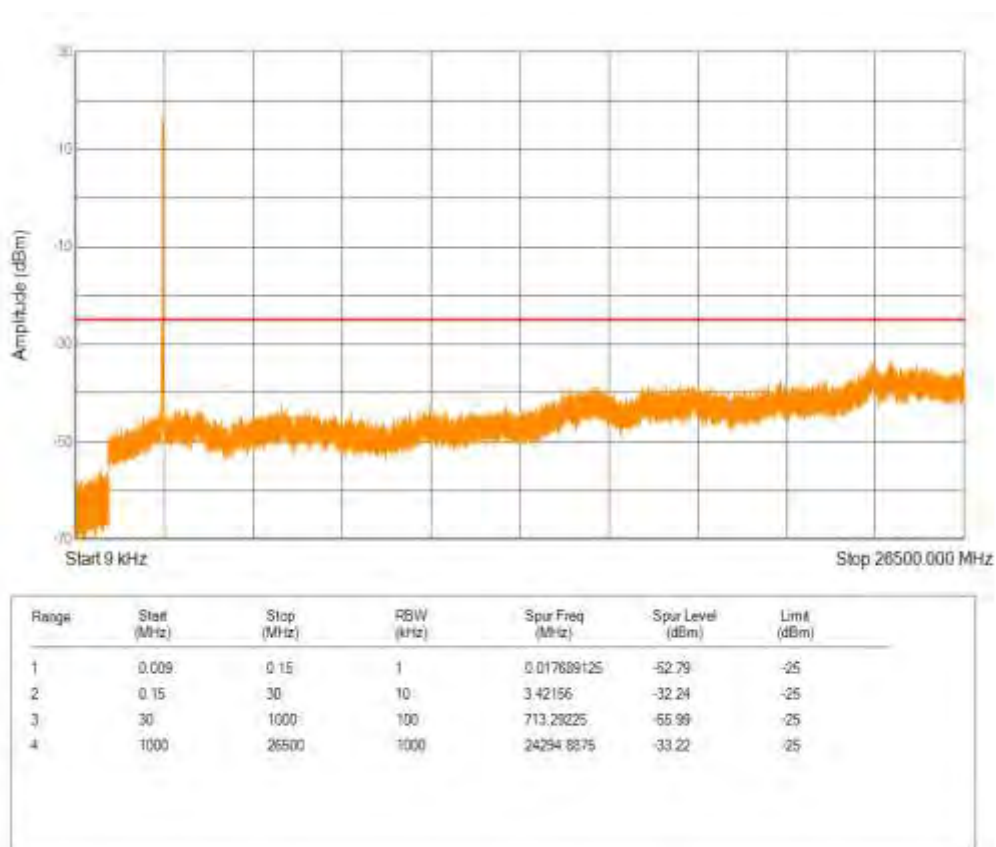
Band41(2555-2655) QPSK BW=20MHz Channel=41140 RB Size=100 Position=#0
