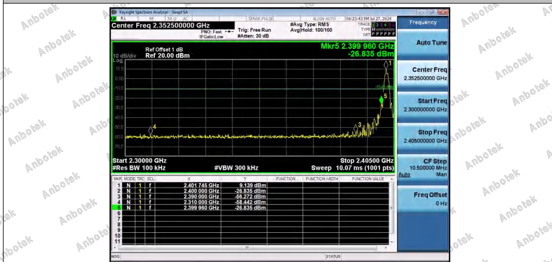
BLE_2M-Ant1-2402-PASS
