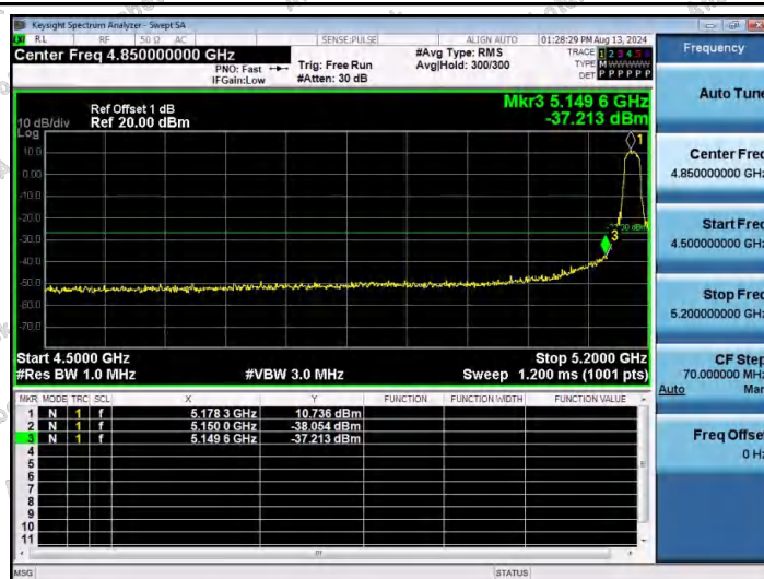
11N20SISO-Ant1-5180-PASS
