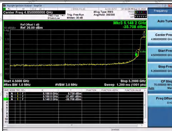
11N40SISO-Ant1-5190-PASS
