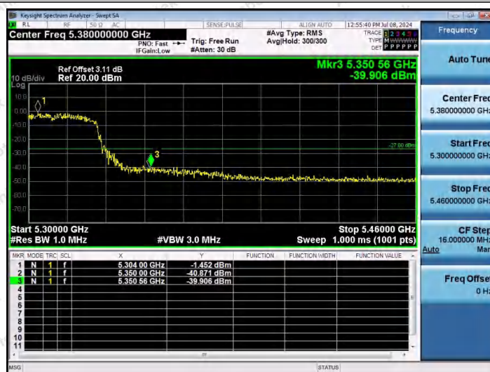
11AC40SISO-Ant1-5310-PASS
