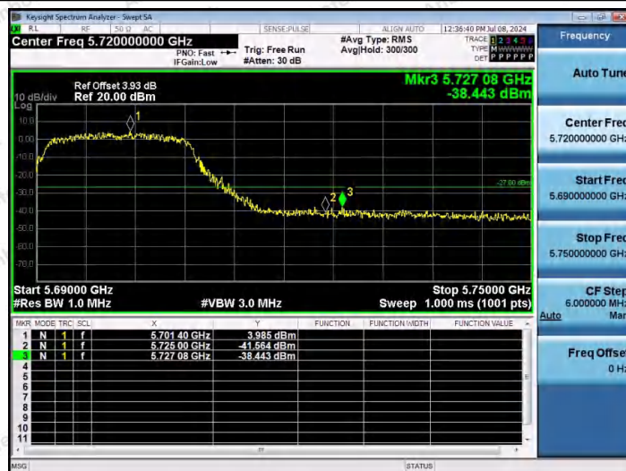
11AC20SISO-Ant1-5700-PASS
