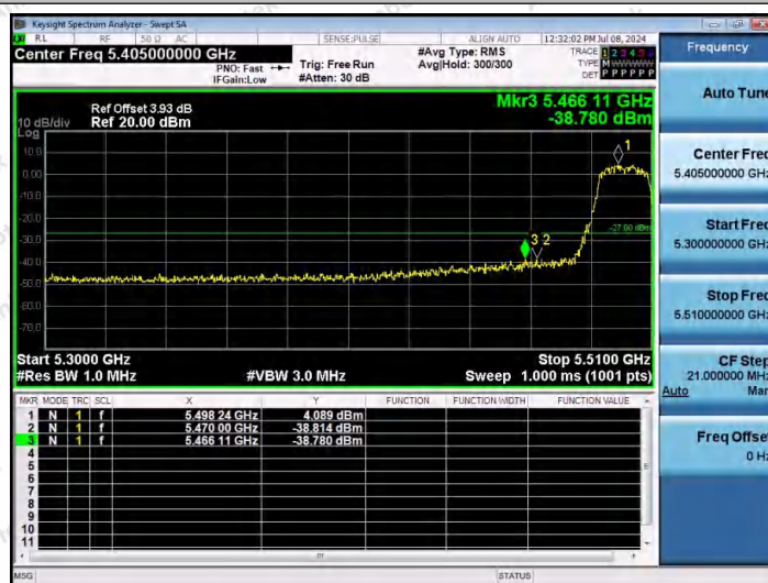
11AC20SISO-Ant1-5500-PASS
