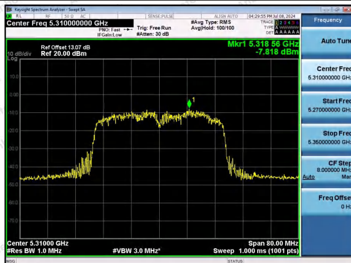
11N40SISO-Ant1-5310-PASS
