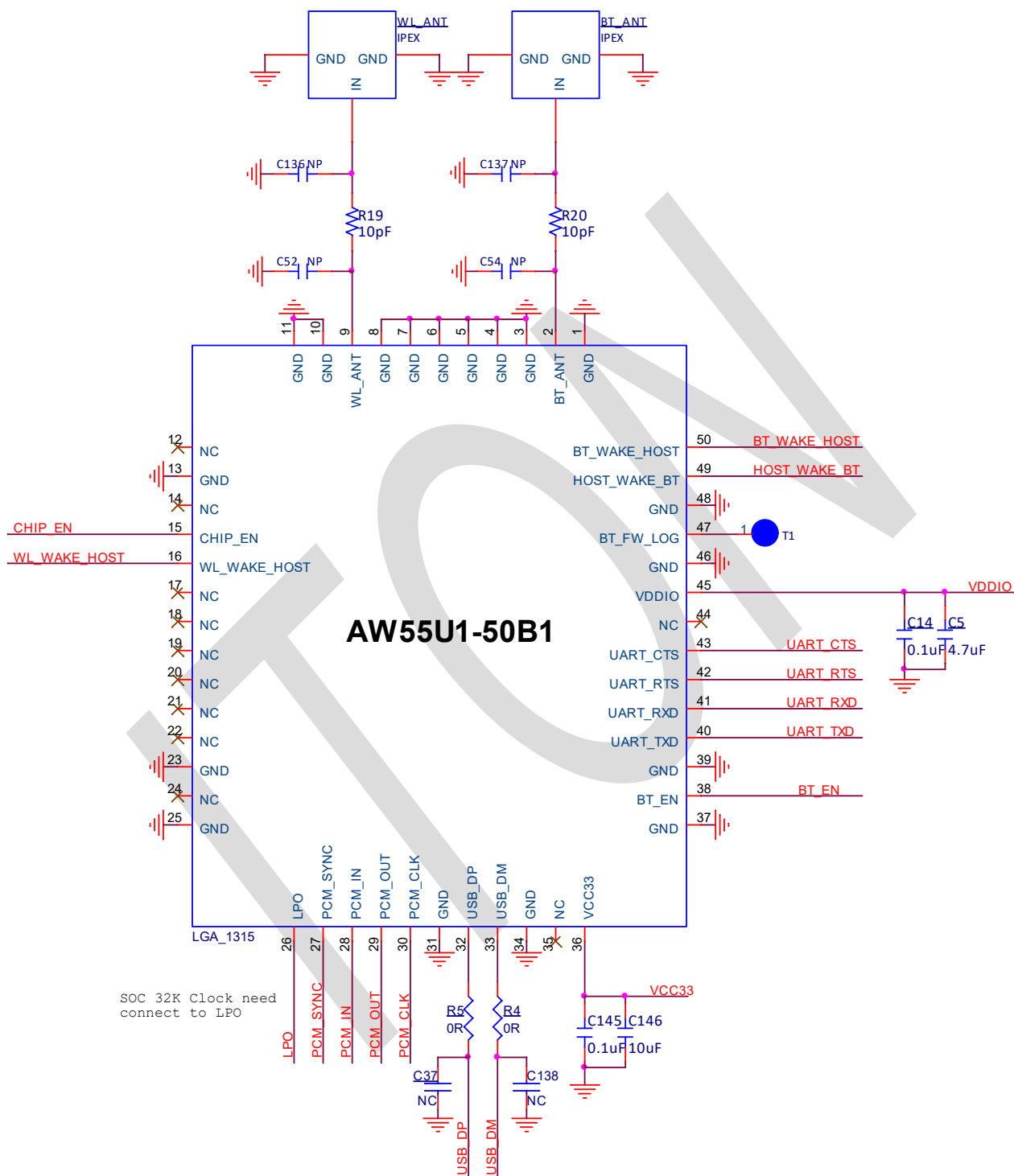
Figure 3. Application Circuit Diagram of AW55U1-50B1
