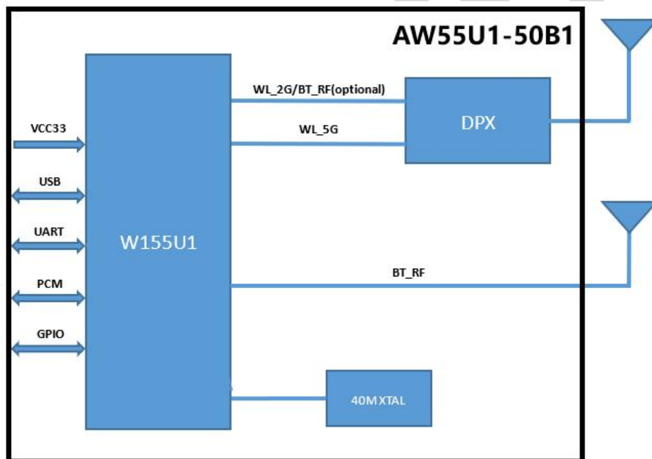
Figure 1. Block Diagram of AW55U1-50B1
