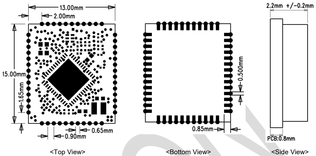
Figure 4. Mechanical Size of AW55U1-50B1
