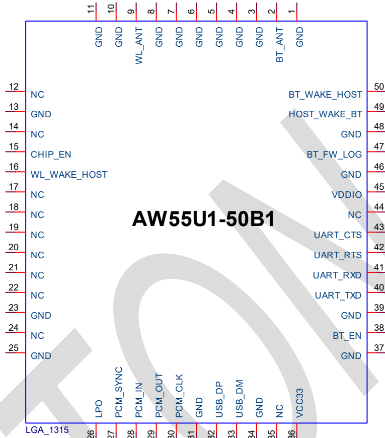
Figure 2.Pin Diagram of AW55U1-50B1
