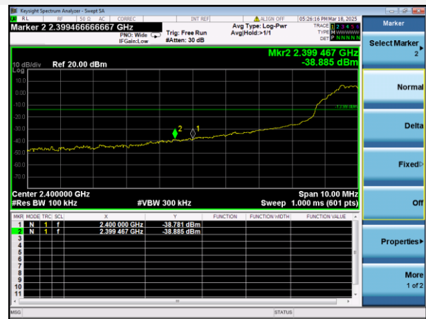
O-QPSK LOW CHANNEL, BAND EDGE
