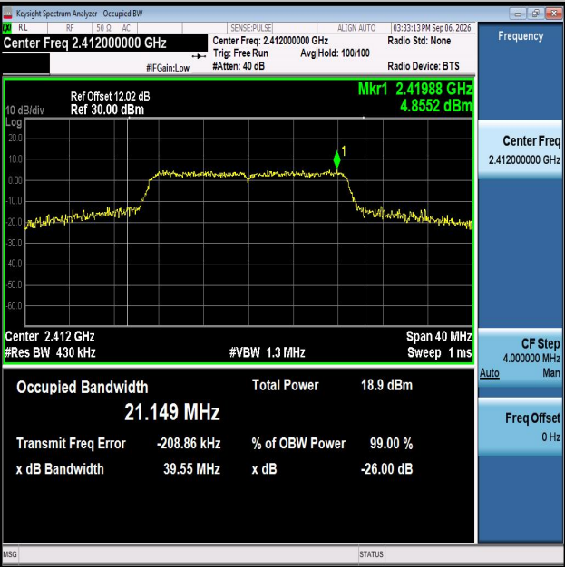
11N20MIMO-Ant2-2412
