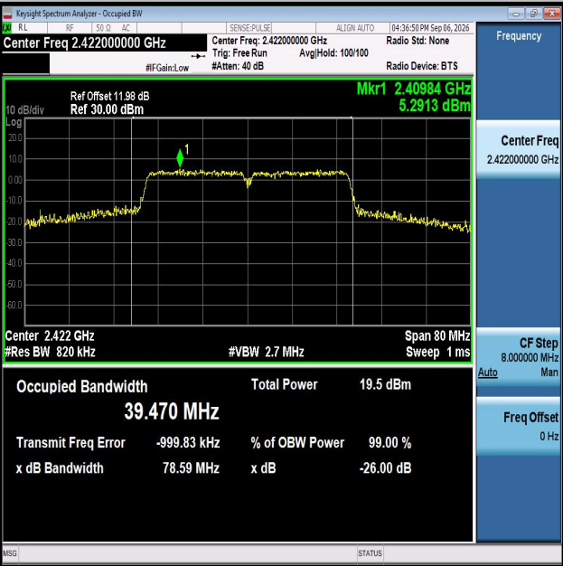
11N40MIMO-Ant2-2422
