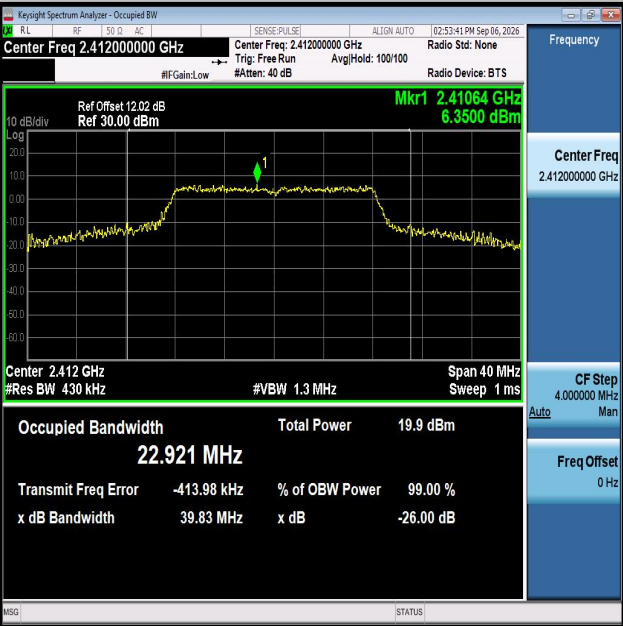
11G-Ant2-2412
