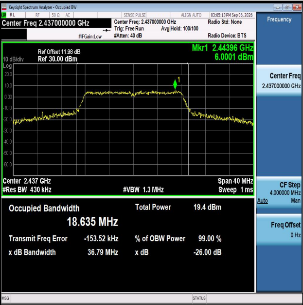
11G-Ant2-2437
