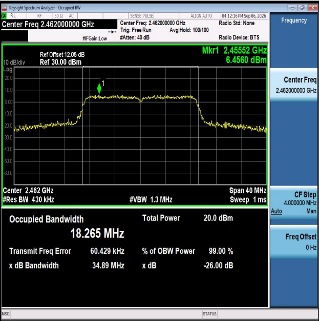
11N20MIMO-Ant2-2462
