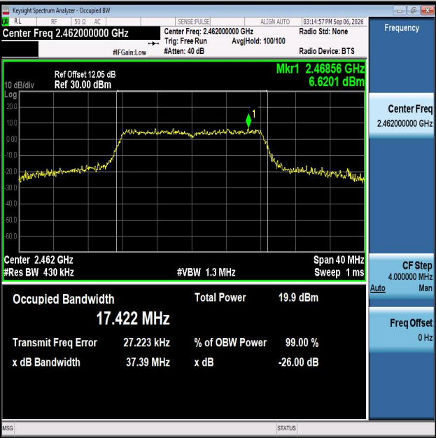
11G-Ant2-2462
